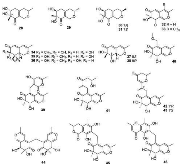
Fig. 3 Chemical structures of austdiol-type azaphilonones (28–46).
