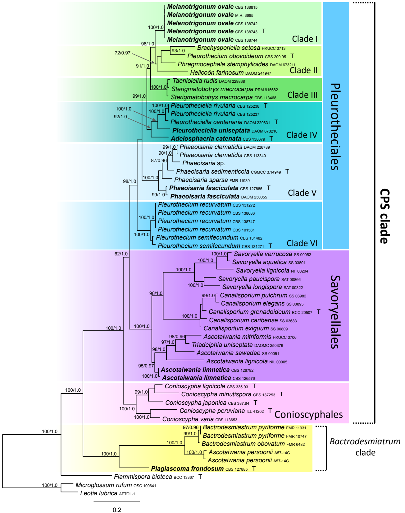
Fig. 2 Multilocus phylogenetic analysis of the ITS-nuc18S-nuc28S-β-tubulin-rpb2-mcm7 sequences of the CPS ( Conioscyphales , Pleurotheciales , Savoriellales ) and Bactrodesmiatrum clades. Phylogram inferred from the ML analysis with RAxML using a GTRCAT model of evolution. Only high branch support is shown at the nodes, ML BS ≥ 70 %, PP ≥ 0.95. Taxa written in bold represent taxonomic novelties.
