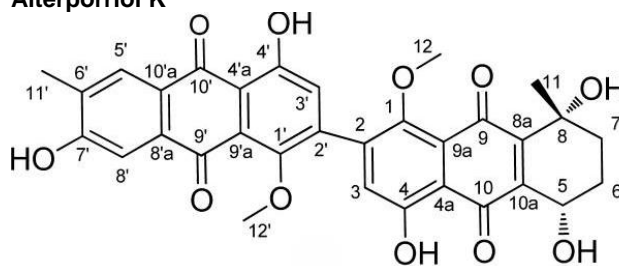
Figure 3: Structure of alterporriol K (Huang et al. , 2011).
