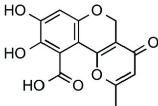
Figure 4: Structure of citromycetin (Mori et al. , 2015).
