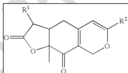
Figure 2: General structure of an azaphilone class pigment (Chen et al. , 2015).
