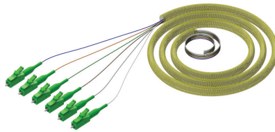
Catalog Number: P6LCA3 6 Fiber LC/APC Pigtail Cable Assembly
