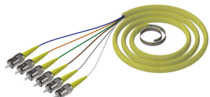
Catalog Number: P6ST3 6 Fiber ST/UPC Pigtail Cable Assembly
