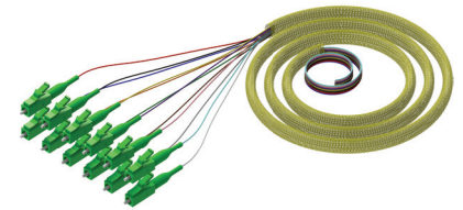
Catalog Number: P12LCA3 12 Fiber LC/APC Pigtail Cable Assembly
