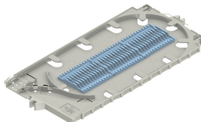
Catalog Number: 80805514 Long – Standard Profile Single Fusion 36 1 Splice Count
