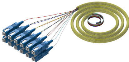
Catalog Number: P12SCU3 12 Fiber SC/UPC Pigtail Cable Assembly
