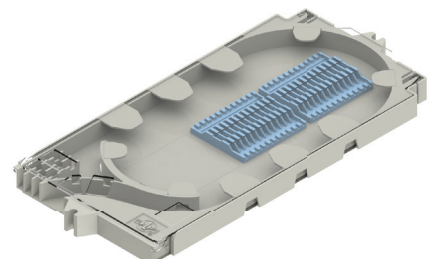
Catalog Number: 80805515 Long – Deep Profile Mass Fusion 144 Splice Count
