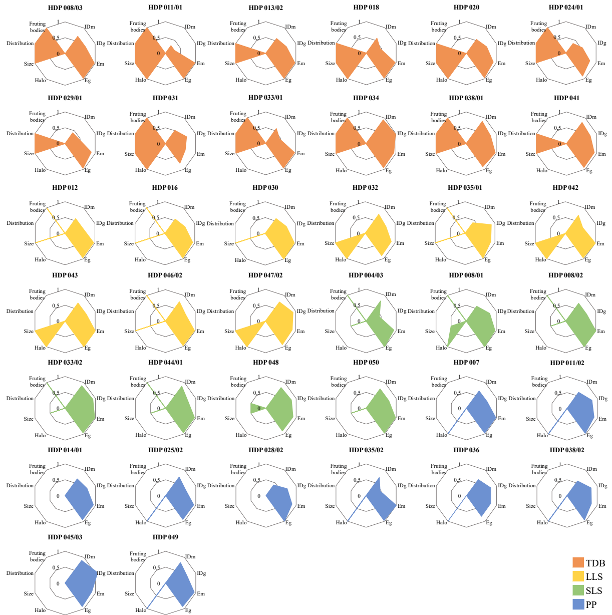
Figure 3.8 Graphical representation of the variation of each foliar lesion morphology and respective fungal community. Variation on foliar lesion morphology (left side of each graph) was assessed considering a three-values scale code (0, 0.5 and 1) for four different characteristics, namely the presence of fructing bodies (no = 0, yes = 1), the distribution along the leaflet or segment (random = 0, specific region = 0.5, at the tip = 1), the size of the foliar lesion (PP = 0, SLS = 0.5, LLS/TDB = 1) and the presence of halo (no = 0, yes = 1). Variation on the fungal community recorded in each foliar lesion (right side of each graph) was assessed through their morphological and genetic index of diversity and evenness, both computed using the Shannon index of diversity applied to the genera richness and its composition and MSP-PCR fingerprintings, respectively. Samples with a relative frequency of isolates < 1% (less than five isolates) were excluded. Colours are according to foliar lesion types. IDm = morphological index of diversity, IDg = genetic index of diversity, Em = morphological evenness, Eg = genetic evenness, TDB = tip die-back, LLS = large leaf spot, SLS = small leaf spot, PP = pinpoints and punctuations.
