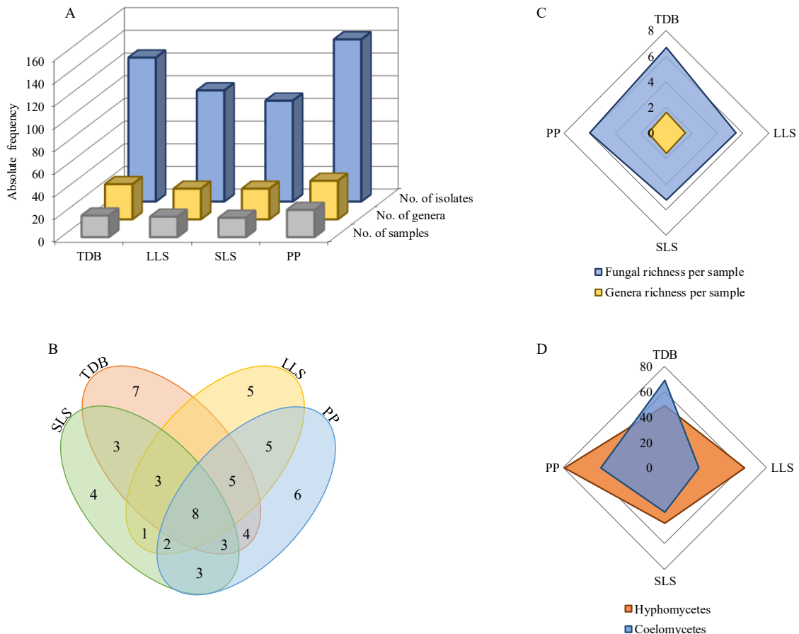
Figure 3.7 General biodiversity patterns of fungal records per foliar lesion type. A. Number of isolates and number of genera yielded, along with the number of samples examined per each foliar lesion type. B. Venn diagram of genera richness by foliar lesion type. C. Graphical representation of fungal richness and genera richness yielded per sample. D. Graphical representation of the absolute frequency of hyphomycetes and coelomycetes isolated from each foliar lesion type. In B colours are according to foliar lesion types. In D colours are according to fungal types. TDB = tip die-back, LLS = large leaf spot, SLS = small leaf spot, PP = pinpoints and punctuations.
