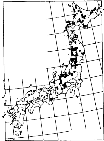
Fig. 13. Distribution of Diphyllia grayi . Modified from Horikawa (1986).
