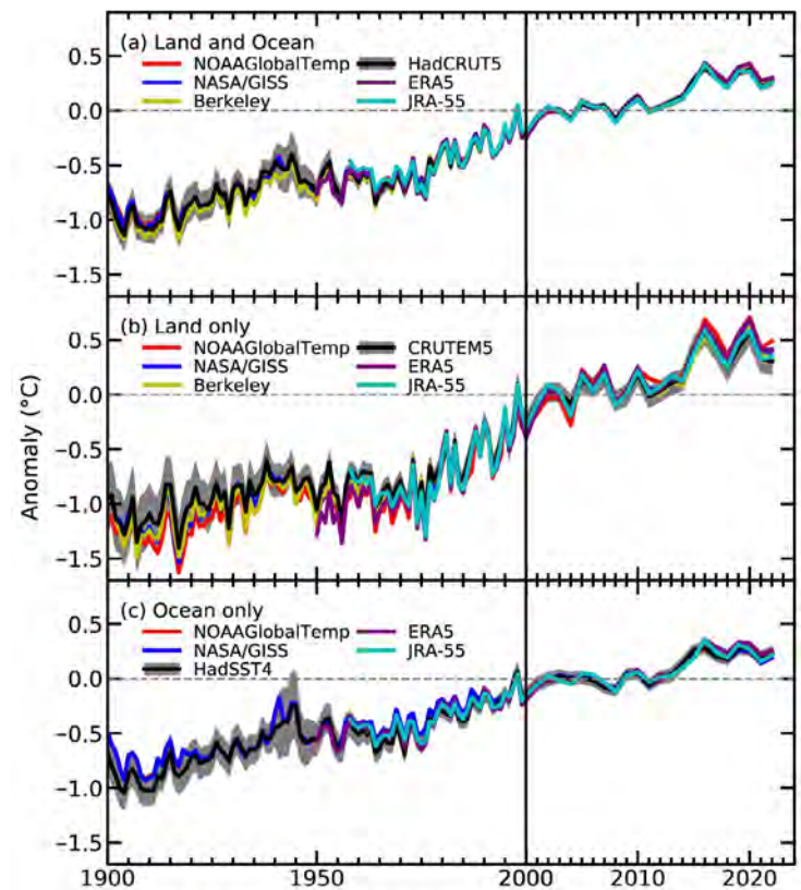
Fig. 2.1. Global average surface air temperature anomalies (°C; 1991–2020 base period) for (a) land and ocean, (b) land only, and (c) ocean only. In situ estimates are shown from the datasets NOAAGlobalTemp (Vose et al. 2021), NASA-GISS (Lenssen et al. 2019), HadCRUT5 (Morice et al. 2021), CRUTEM5 (Osborn et al. 2021), HadSST4 (Kennedy et al. 2019), and Berkeley (Rhode and Hausfather 2020). The 95% confidence ranges are also shown for HadCRUT5, CRUTEM5, and HadSST4. Reanalyses estimates are shown from the datasets ERA5 (Hersbach et al. 2020) and JRA-55 (Kobayashi et al. 2015).
