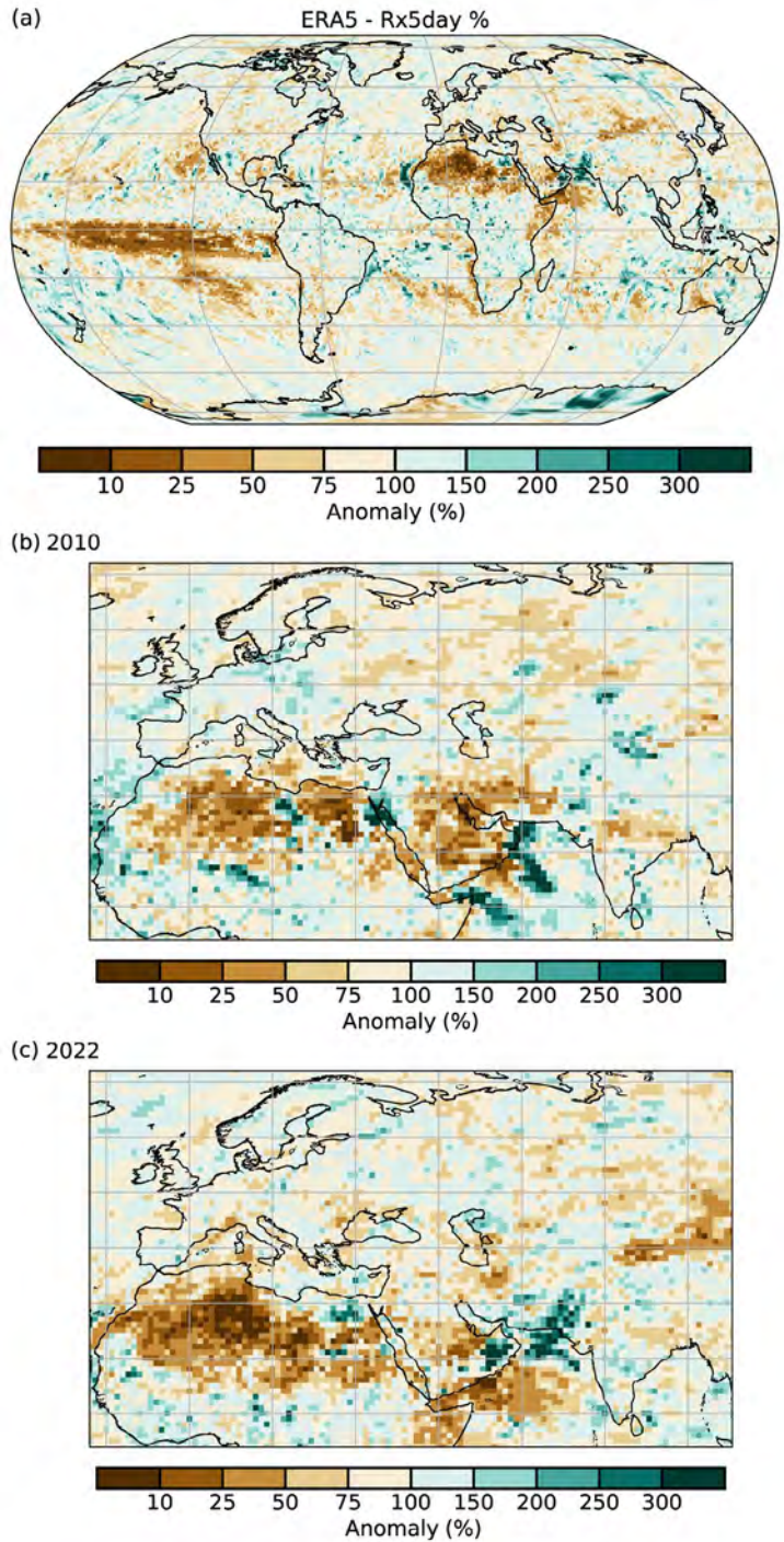
Fig. 2.30. Annual maximum five-day precipitation (Rx5day) as a percentage of the 1991–2020 average for (a) the globe and over Europe and South Asia in (b) 2010 and (c) 2022. (Source: ERA5.)
