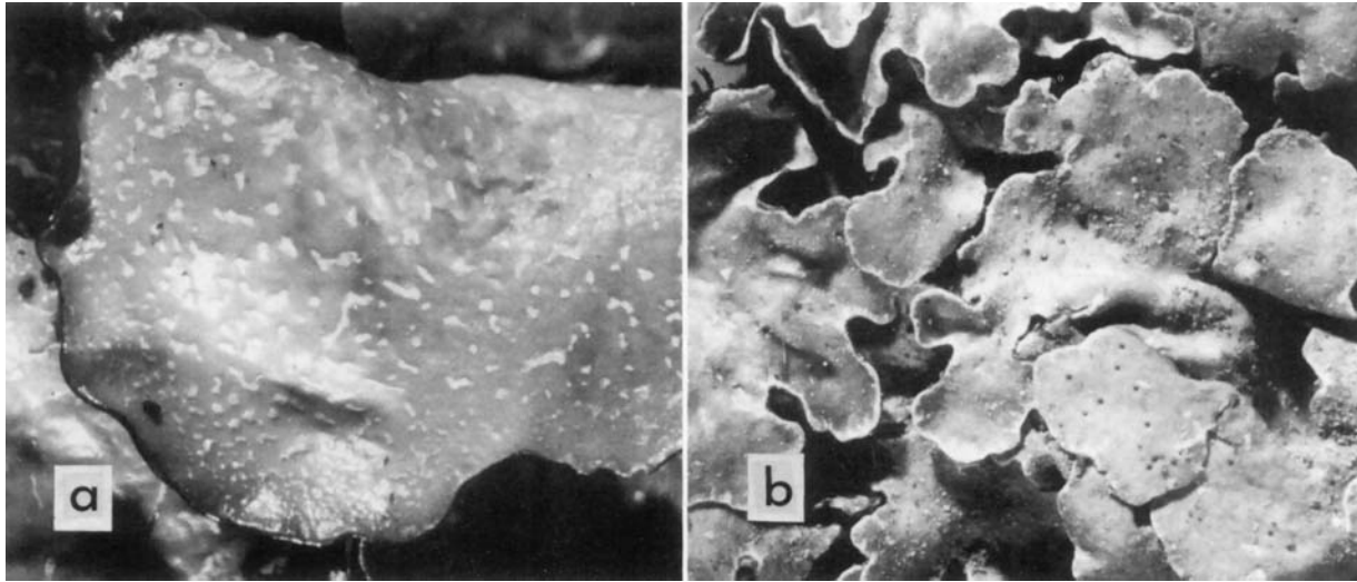
FIGURE 8.—Orientation of pseudocypellae in Parmelia species: a, P. tenuirima (James 488 pp.); b, P. testacea (Hale 65112). (All \times 8.5 .)
