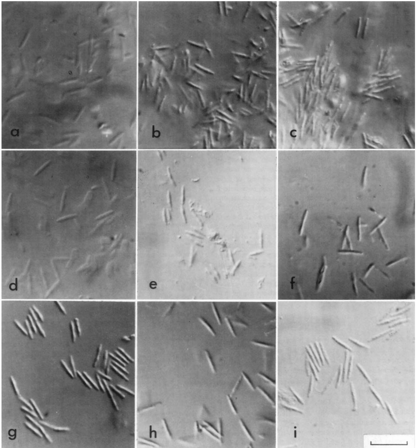
FIGURE 12.—Conidia of Parmelia species: a, P. cochleata (isoelectotype in US); b, P. cunninghamii (Santesson 7814); c, P. discordans (Kjellm s.n.); d, P. testacea (James 561); e, P. erumpens (Hale 43657); f, P. marmorata (Nakanishi 2811); g, P. omphalodes (Hale 18851); h, P. saxatilis (Hale 49288); i, P. sulcata (Hale 49675a). (Scale in i = 10 \mu m.)
