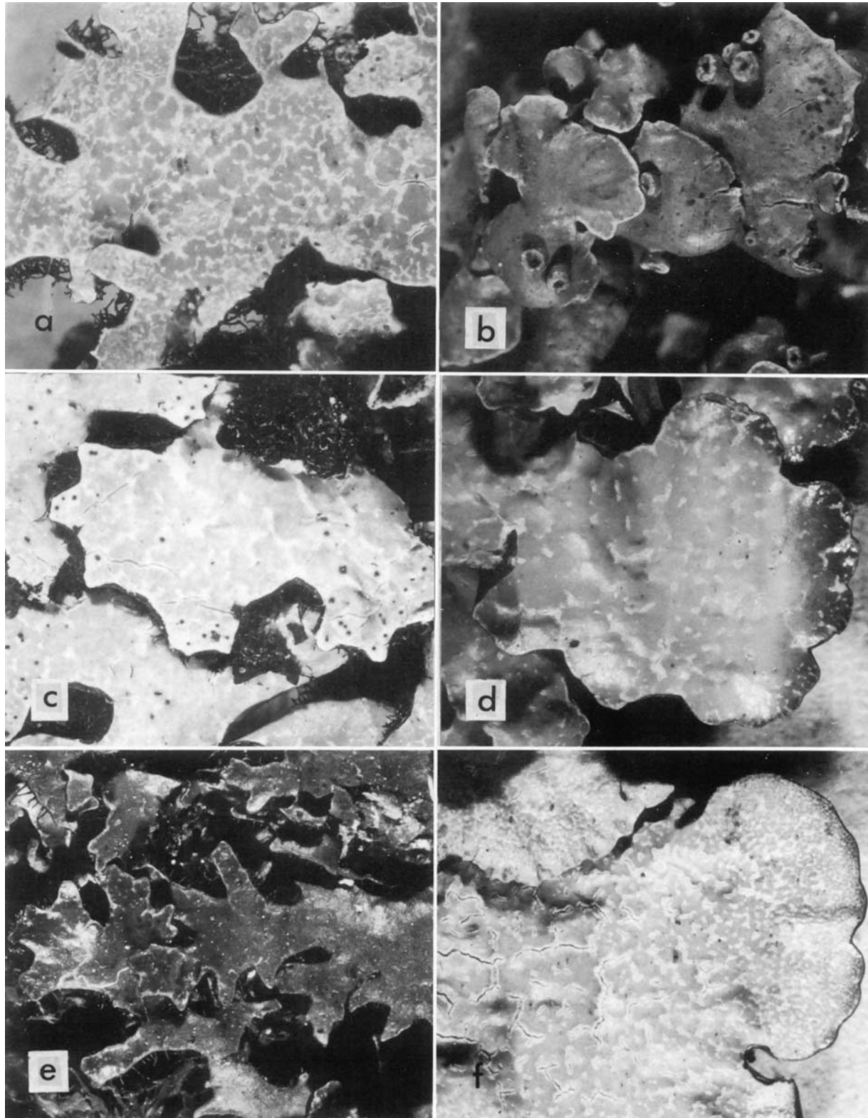
FIGURE 2.—Orientation of pseudocyphellae in Parmelia species: a, P. adaugescens (Asahina s.n.); b, P. cochleata (isolecotype in US); c, P. crambidiocarpa (Hale, 65541); d, P. cunninghamii (Santesson 6792); e, P. discordans (Issin s.n.); f, P. erumpens (Hale 43876). (All \times 8.5 .)
