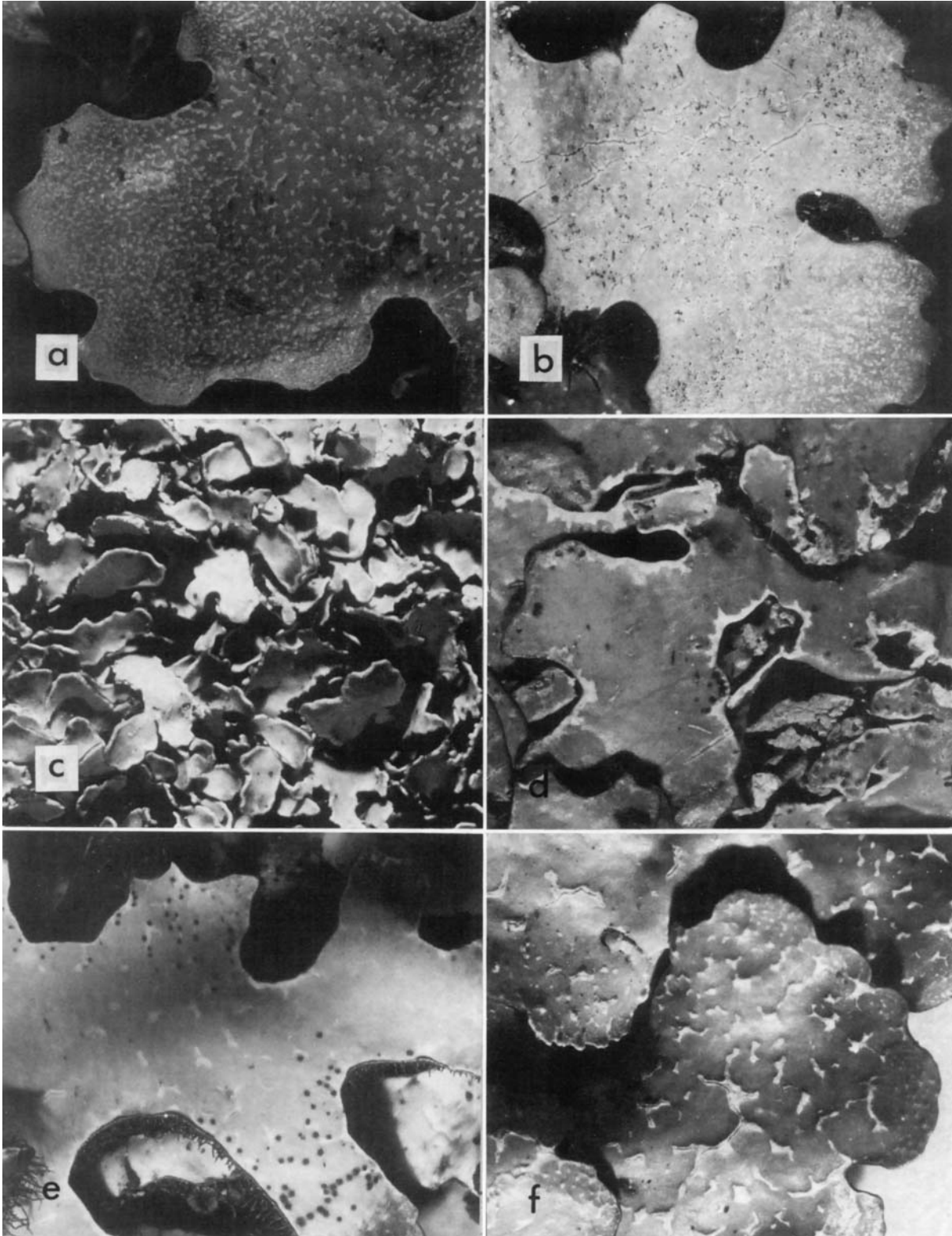
FIGURE 4.—Orientation of pseudocyphellae in Parmelia species: a, P. marmorata (Kurokawa 58062); b, P. meiophora (Poelt L-151); c, P. neodiscordans (holotype in US); d, P. niitakana (Hsu 1374); e, P. norcrambidiocarpa (holotype in US); f, P. novae-zelandiae (Hale 66232). (All \times 8.5 .)
