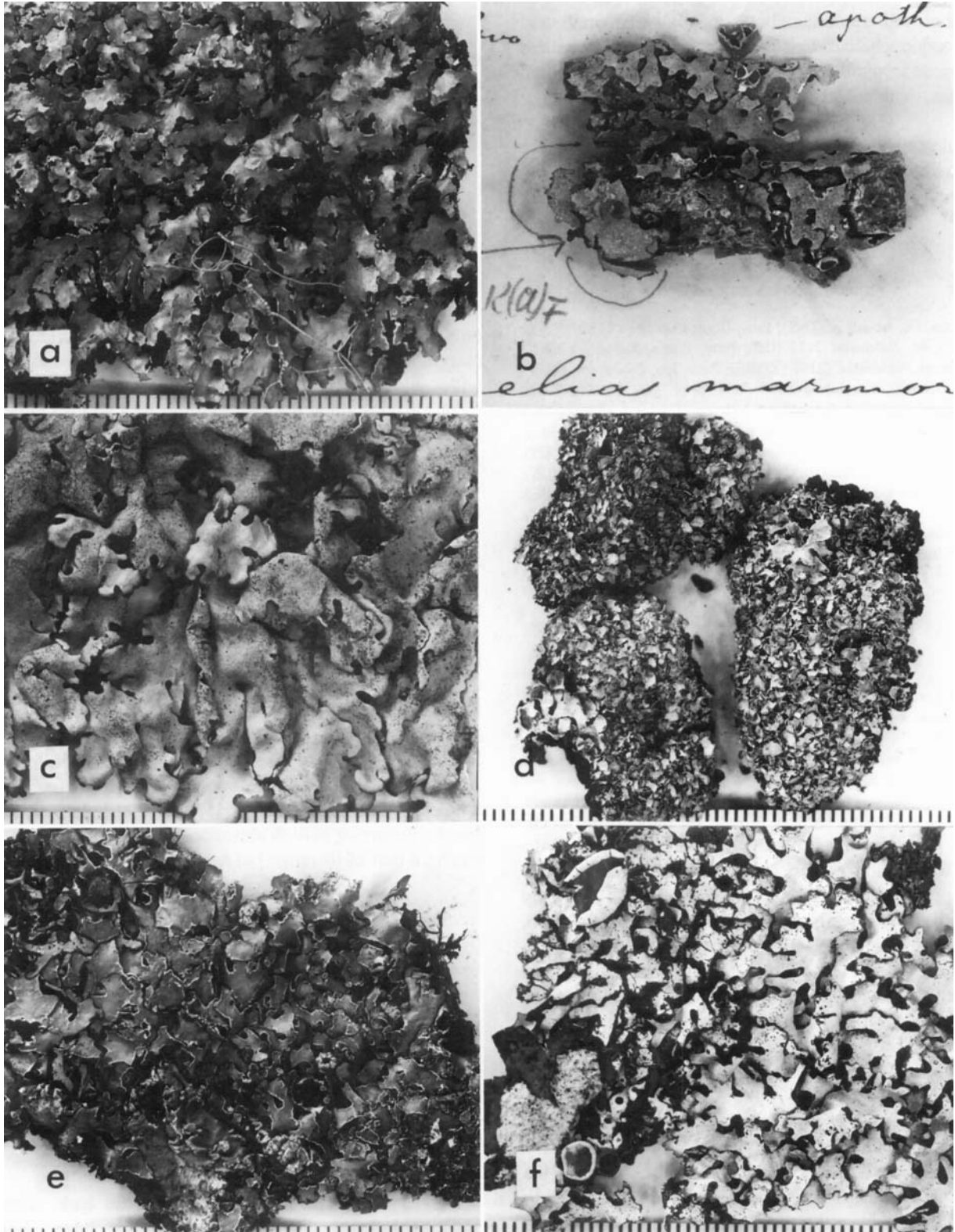
FIGURE 17.—Species of Parmelia : a, P. laevior (Hale 29357); b, P. marmor (lectotype in H); c, P. meiophora (Poelt L-151); d, P. neodiscordans (holotype in US); e, P. niitakana (Hsu 1374); f, P. norcrambidiocarpa (holotype in US). (Scales in mm.)
