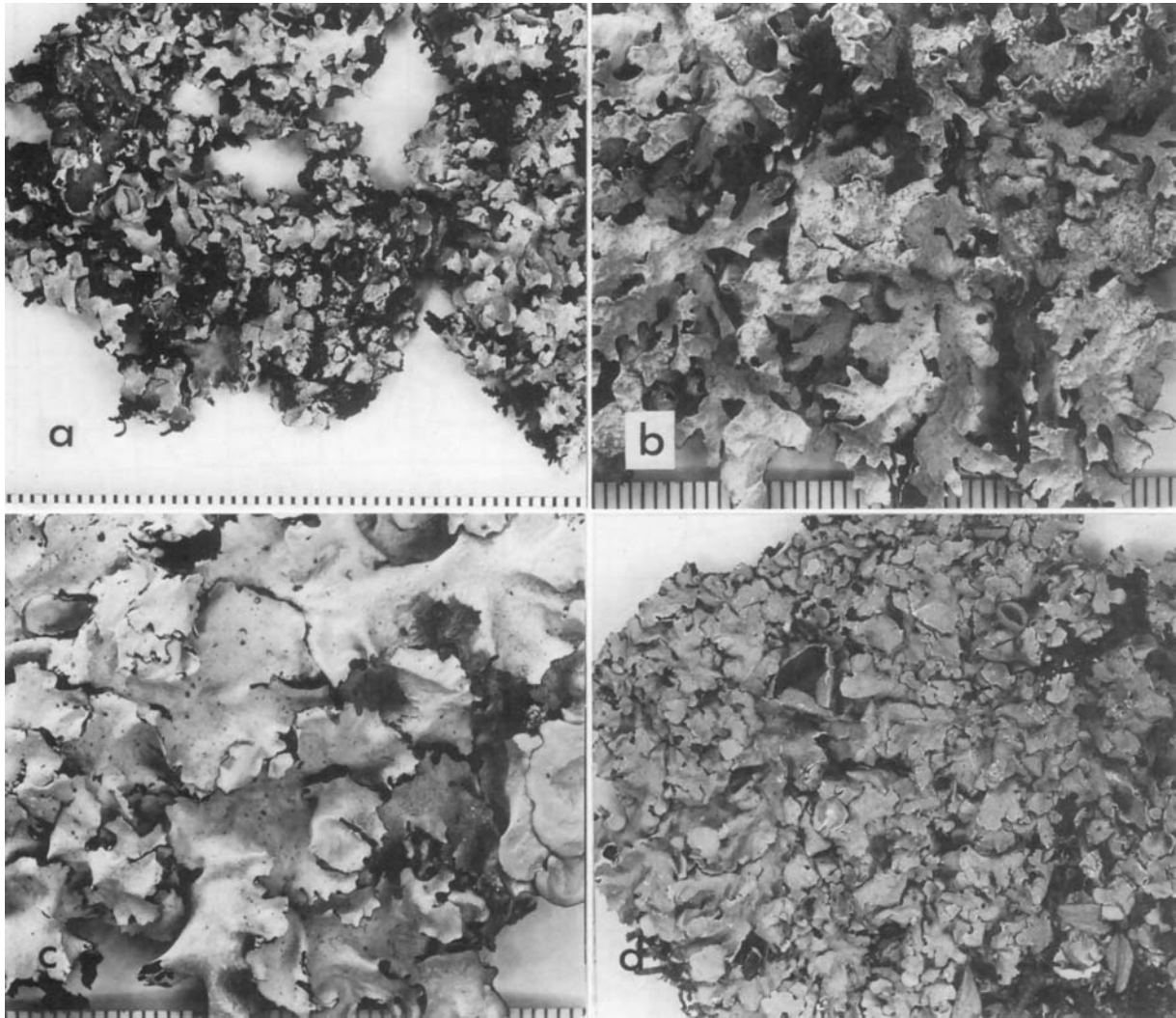
FIGURE 23.—Species of Parmelia : a, P. substestacea (holotype in US); b, P. sulcata (Kjellmert s.n.); c, P. tenuirima (James 488 pp.); d, P. rudior (type of P. erimis in H). (Scales in mm.)
