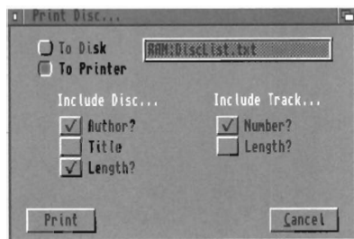
AsimTunes – Print Disc
