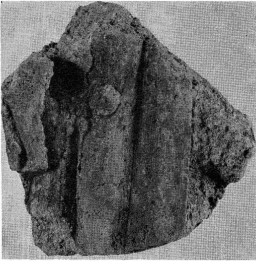
FIG. 4. ? Freycinetia mariannensis , portion of central section of leaf, showing venation.
