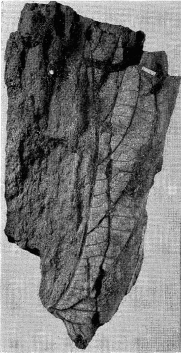
FIG. 11. Trema argentea , portion of leaf, showing venation.
