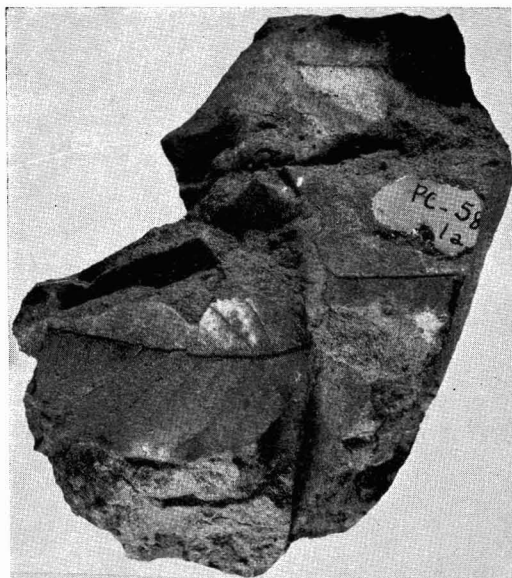
FIG. 13. Tristiropsis obtusangula , impression of leaflet, showing texture and venation.
