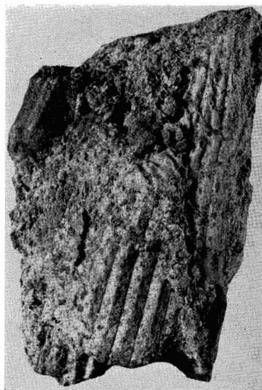
FIG. 10. ? Spatoglottis micronesiaca , portion of leaf blade showing plication.
