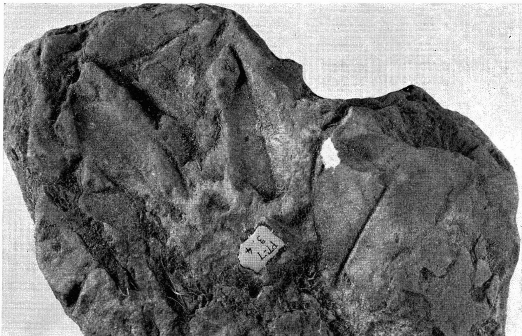
FIG. 12. Aglaia mariannensis , impression on right, base of large leaflet, that on left, possibly one of smaller leaflets. Elaeocarpus joga , impression in center, leaf blade and petiole.
