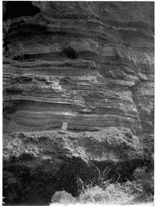
FIG. 2. Tuff overlying lava and underlying tuff-breccia at the west end of the caldera rim. Plant impressions were collected from the tuff below and interbedded with the dark colored cindery layers in the upper part of the picture. The hole in the cindery layer was probably formed by decay of a tree trunk that had been buried by the ash. The sides of similar holes elsewhere commonly retain impressions of tree bark. A deformed tuff layer near the center of the picture may represent the soil horizon in which the plants grew.
