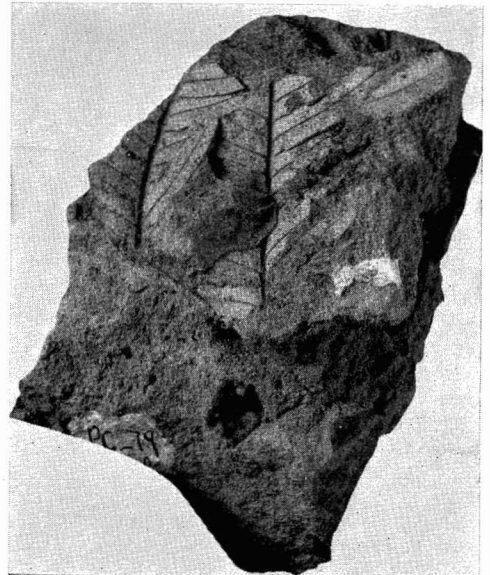
FIG. 3. Pteris quadriaurita , fragmentary impression of frond showing portion of rachis, pinnae, with pinnules.
