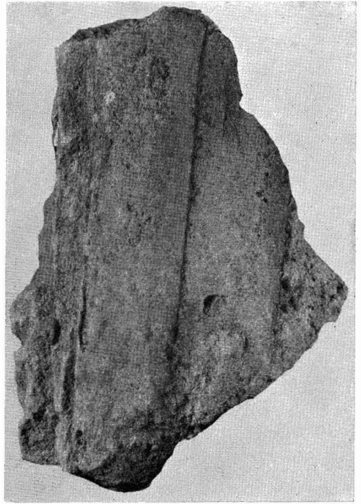
FIG. 5. Pandanus tectorius , portion of central section of leaf.
