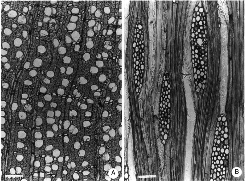
Fig. 2.—A, Myodocarpus elegans var. gracilis , Lowry 3377A , transverse section: axial parenchyma diffuse-in-aggregates and diffuse, very thick-walled fibers.—B, M. traxinifolius , Lowry 3679 , tangential section: multiseriate rays up to 5 rows wide, radial canal. Scale bars = 100 µm.
