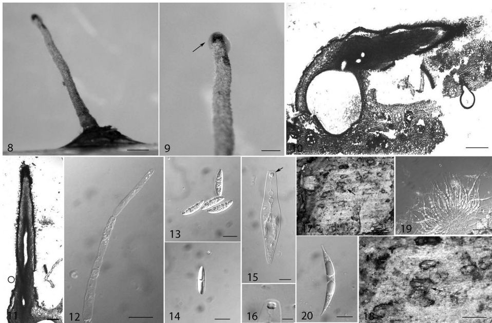
Figs 8-16. Pseudohalonectria miscanthicola (from holotype). 8. Ascoma partially immersed in the host surface. 9. Apical portion of neck showing deposition of ascospores/asci (arrowed). 10. Section of an ascoma. 11. Vertical section of neck. 12. Paraphyses. 13, 14. Ascospores. 15. An empty ascus showing an apical refractive ring (arrowed). 16. A non-amyloid (refractive) apical ring. Figs. 17-20. Oxydothis oraniopsis . 17, 18. Surface view of fruiting structures on host (arrowed). 19. Squash mount of contents of an ascoma. 20. An ascospore showing long narrow processes.
