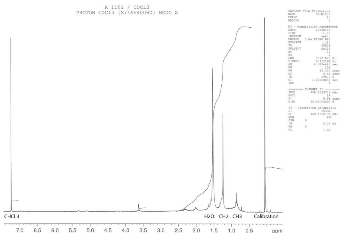
Figure III.7. Result of the NMR analysis showing the presence of \text{CH}_3 and \text{CH}_2 for Riv. PPB 126.
