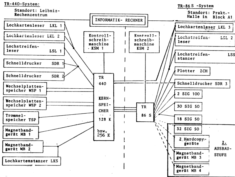
TR 440 Konfiguration (1972)
