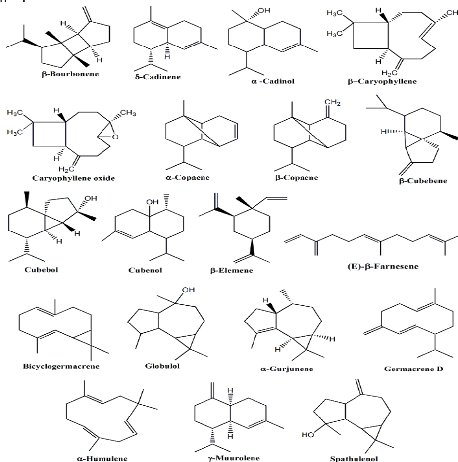
Figure 1b: Sesquiterpenes and oxygenated sesquiterpenes identified from essential oil of O. killandscharicum
