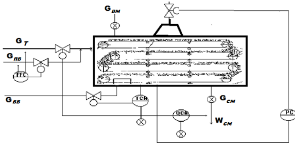
3-picture. Scheme for automation of the drying process
