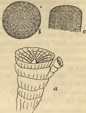
Lonsdaleia : a. old branch exterior and terminal cups and young one growing from the side. b. Transverse section showing the three areas and a bud (x) growing in the outer one. c. Vertical section.
