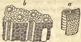
Fistulipora : a. mode of growth, nat. size, enveloping a crinoid stem. b. magnified surface and section.
