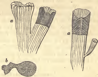
Recent Lithodendron . a. Mode of growth and vertical section. b. Horizontal section.
