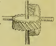
Spiral-wheel.
