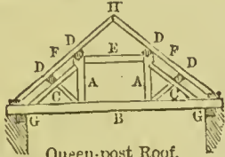
Queen-post Roof.
