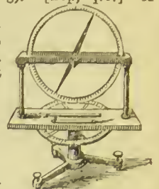
Dipping-needle.
