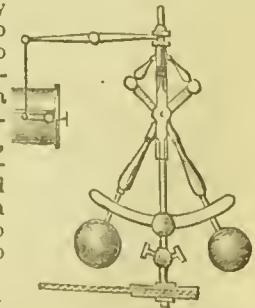
Governor.
