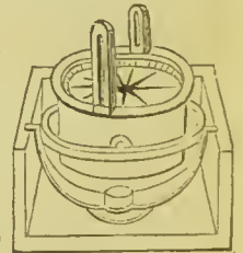
Azimuth.
