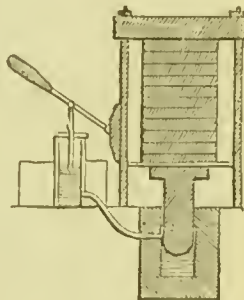
Hydraulic press.
