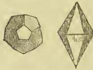
Dodecahedrons.
