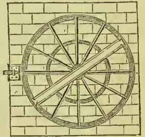
Mural circle.
