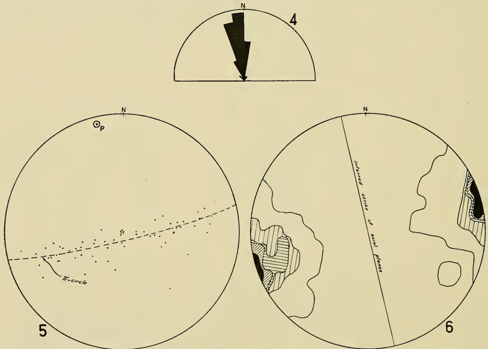
Fig. 4. Rose diagram of trends of 69 axial traces of folds (derived from maps in Crook, 1961 a, b ).
