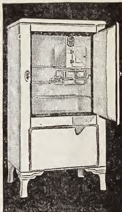
The Guardian—Model 71: Capacity, 7.53 cu. ft.; Shelf area, 11.35 sq. ft.; Ice, 4 trays, 21 cubes each, total 84. Finish: Exterior and Interior, Porcelain. Height, with 8½ in. legs, 61¼ in.; width, 32¾ in.; depth, 25¾ in. Watervoir shown in this model is extra equipment.
