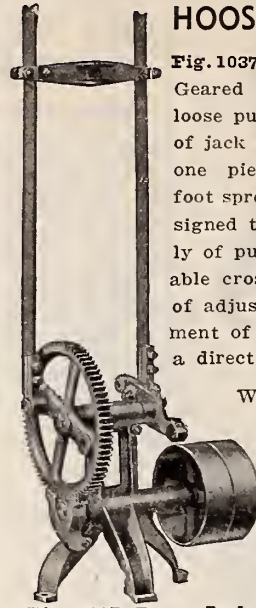
Fig. 1037, Pump Jack
