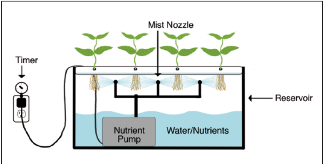
Figure 6. Diagrammatic representation of an aeroponic minituber propagation system. (Diagram © Green desert.org, With permission)
