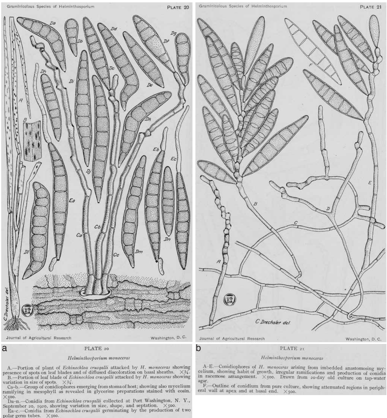
Fig. 7 Original drawing of Helminthosporium monoceras (reproduced from Drechsler 1923). a. From natural substrate Echinochloa crus-galli ; b. from culture.
