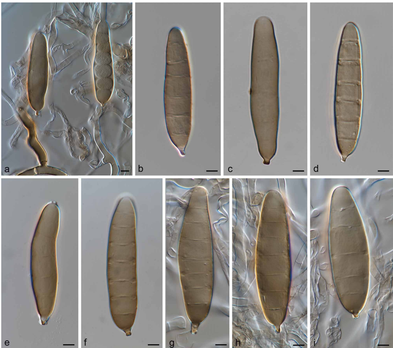
Fig. 12 Exserohilum protrudens (BRIP 14816). a. Conidiophore and conidia; b–i. conidia. — Scale bars: 10 μm.
