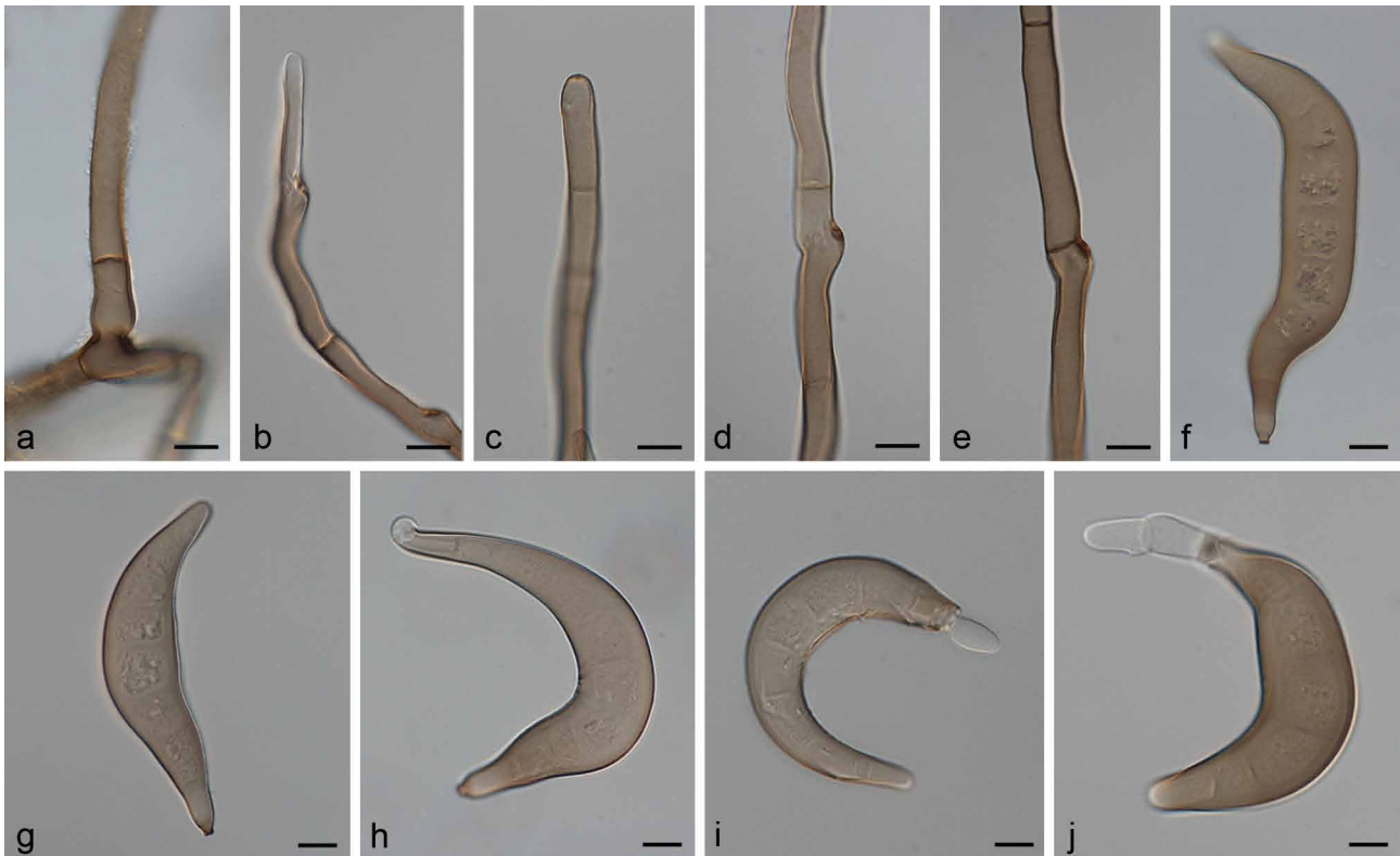
Fig. 23 Exserohilum oryzinum (IMI 152682 holotype). a. Conidiophore with a swelling base; b–e. conidiogenous cells; f–j. conidia. — Scale bars: 10 \mu m.
