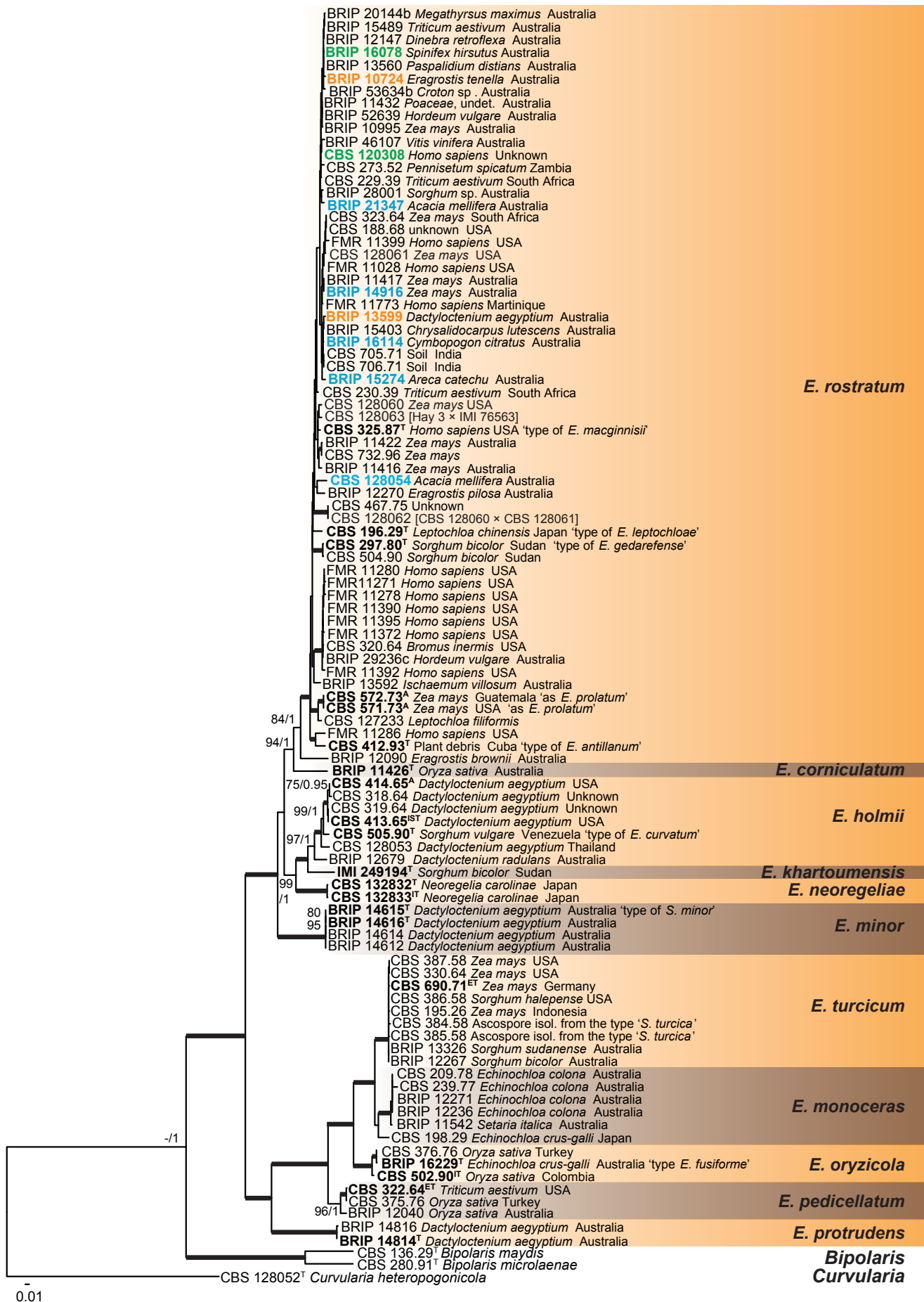
Fig. 2 Phylogenetic tree inferred from a RAxML analysis based on a concatenated alignment of ITS, act , gapdh , his , rbp2 , tef1 and tub2 sequences of Exserohilum s.str. The bootstrap support values and Bayesian posterior probabilities are given at the nodes (MLBS/BPP). Clades with 100 % MLBS and 1 BPP are indicated by thickened lines. In the E. rostratum clade in green font are indicated taxa previously identified as E. macginnisii , in blue identified as E. longirostratum , in orange as E. holmii . Ex-type, ex-isotype, ex-neotype and ex-epitype strains are indicated in bold. The tree was rooted to Bipolaris maydis CBS 136.29, B. microlaenae CBS 280.91 and Curvularia heteropogonicola CBS 128052.
