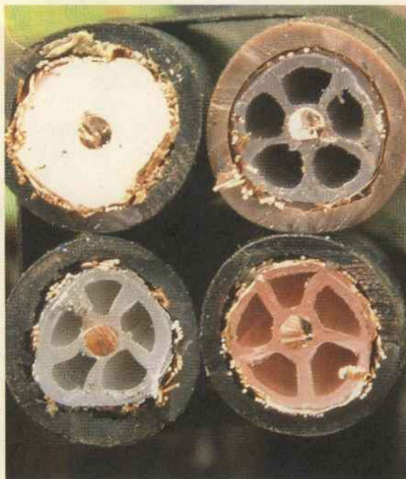
Fig. 2: Different types of dielectric. Top left, foam dielectric used in type B cable; top right, semi-airspaced used in type D cable; bottom left semi-airspaced used in type C cable; bottom right semi-airspaced used in type A cable.
