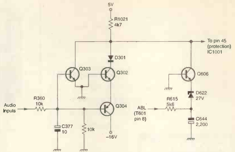
Fig. 46: The audio-output and beam-current monitoring circuitry.
