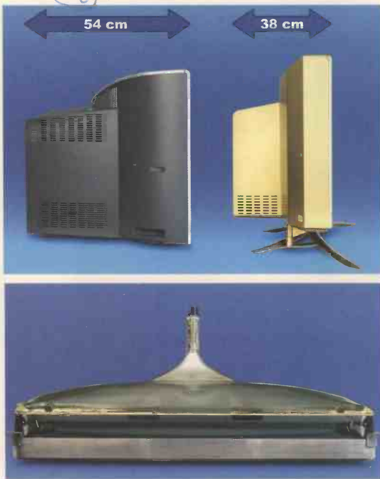
Photo 2: The LG.Philips 32in. widescreen Cybertube+ SuperSlim tube also enables the depth of a set to be reduced to 38cm, giving it a clearly slim-line appearance.
