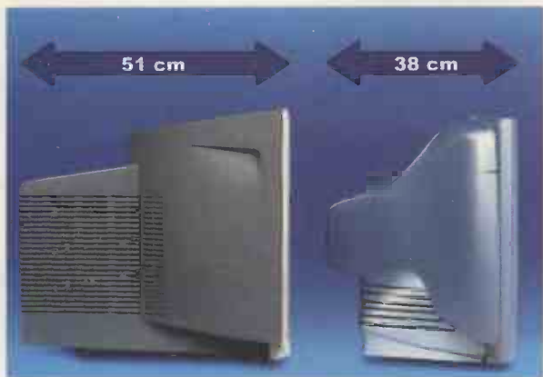
Photo 1: Use of the new LG.Philips 21in. Cybertube+ SuperSlim tube enables the depth of a typical 21in. real-flat 4:3 format TV set to be reduced by 13cm, to about 38cm.
