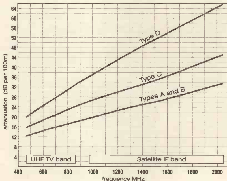
Fig. 3: Comparison of signal attenuation per unit length with different types of cable.
