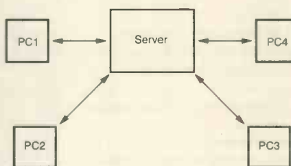
Fig. 2: Server-client networking.
