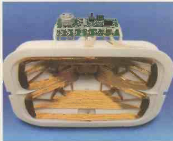
Photo 4: The double-mussel rectangular-coil deflection yoke assembly developed for the 32in. widescreen Cybertube+ SuperSlim CRT.
