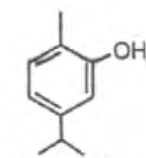
Carvacrol
