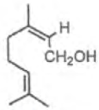
Nerol
