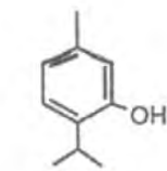
Timol
