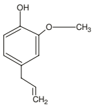
Eugenol
