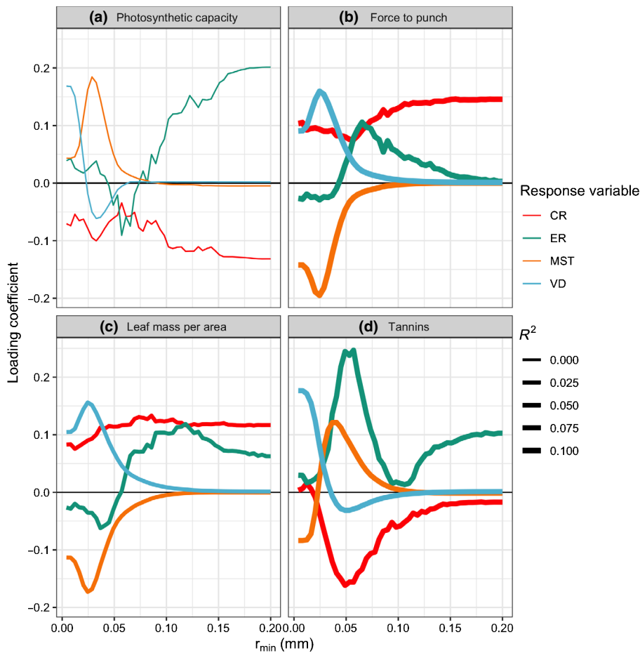
Fig. 5 Summaries of partial least squares (PLS) models predicting leaf functional traits from elongation ratio (ER), circularity ratio (CR), vein density (VD), and minimum spanning tree ratio (MST) across scales, at each value of minimum vein size ( r_{\min} ). Each facet indicates a model with a different leaf functional trait: (a) photosynthetic capacity, (b) force to punch, (c) leaf mass per area and (d) tannins fraction. Colored lines indicate standardized effects of each multiscale statistic at each spatial scale. Thicker colored lines indicate models with higher R^2 . Loading coefficients reflect the first PLS component only.
