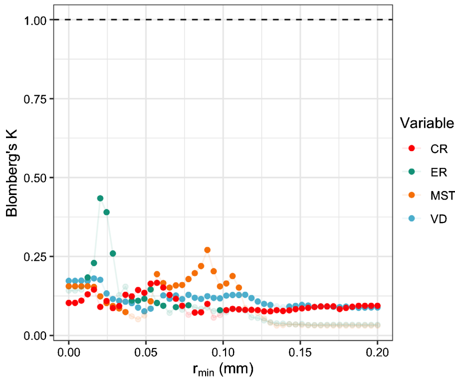
Fig. 7 Blomberg's K statistic of phylogenetic conservatism for elongation ratio (ER), circularity ratio (CR), vein density (VD), and minimum spanning tree ratio (MST) at each value of minimum vein size ( r_{\min} ) (colored dots). Values of 1 (dashed horizontal black line) indicate Brownian trait evolution; values < 1 indicate more rapid evolution than under Brownian trait evolution. Points are solid if significantly different from 1 ( P < 0.05 ) and transparent otherwise.
