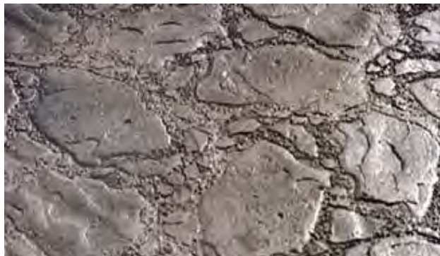
Random Stone, FM-700 29.125" x 29.125" (73.97 x 73.97 cm) Red, Yellow and Blue. Matching skin/touch-up wheel: Rough Stone/ FM-6520 Joint size 1/4"-3/4" wide, 3/8" deep Stone size 7"-11 1/2" wide, 10"-15" long
