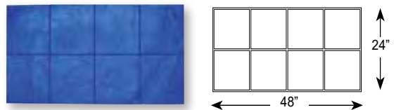
12" x 12" Slate - 1/4" Joint, TM-600 24" x 48" (60.96 x 121.92 cm) Pattern: A Matching skin/touch-up wheel: Slate/ FM-6550 Joint size \frac{3}{8} "- \frac{1}{2} " wide, \frac{1}{4} " deep Stone size 12" square
