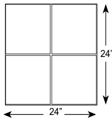
12" x 12" Cut Stone, FM-300 S/O 24" x 24" (60.96 x 60.96 cm) Red Matching skin/touch-up wheel: Smooth Slate/ FM-6510 Joint size \frac{1}{4} "- \frac{3}{4} " wide, \frac{3}{8} " deep Stone size 12"
