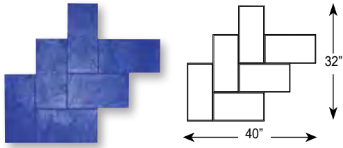
Herringbone Slate, FM-3550 S/O 32" x 40" (81.28 x 101.6 cm) Blue Matching skin/touch-up wheel: Smooth Slate/ FM-6550 Joint size \frac{1}{8} "- \frac{3}{8} " wide, \frac{3}{8} " deep Stone size 8" wide, 16" long
