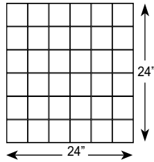
4" x 4" Slate Sets, FM-200 S/O 24" x 24" (60.96 x 60.96 cm) Red Matching skin/touch-up wheel: Smooth Slate/ FM-6510 Joint size \frac{1}{8} "- \frac{1}{4} " wide Stone size 4"
