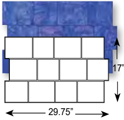
London Cobble, FM-540 S/O 17" x 29.75" (43.18 x 75.56 cm) Blue Matching skin/touch-up wheel: Slate/ FM-6510 Joint 1/8"-1/4" wide, 1/4" deep Stone size 5 1/2"-5 3/4" wide, 6"-8" long
