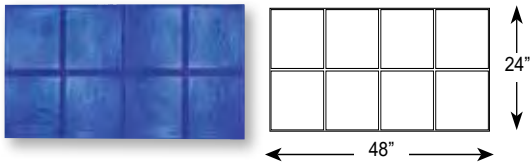
12" x 12" Mexican Tile, TM-1400 24" x 48" (60.96 x 121.92 cm) Pattern: A Matching touch-up wheel: FM-6570 Joint size 3/4" wide, 1/4" deep Tile size 11 1/4" square
