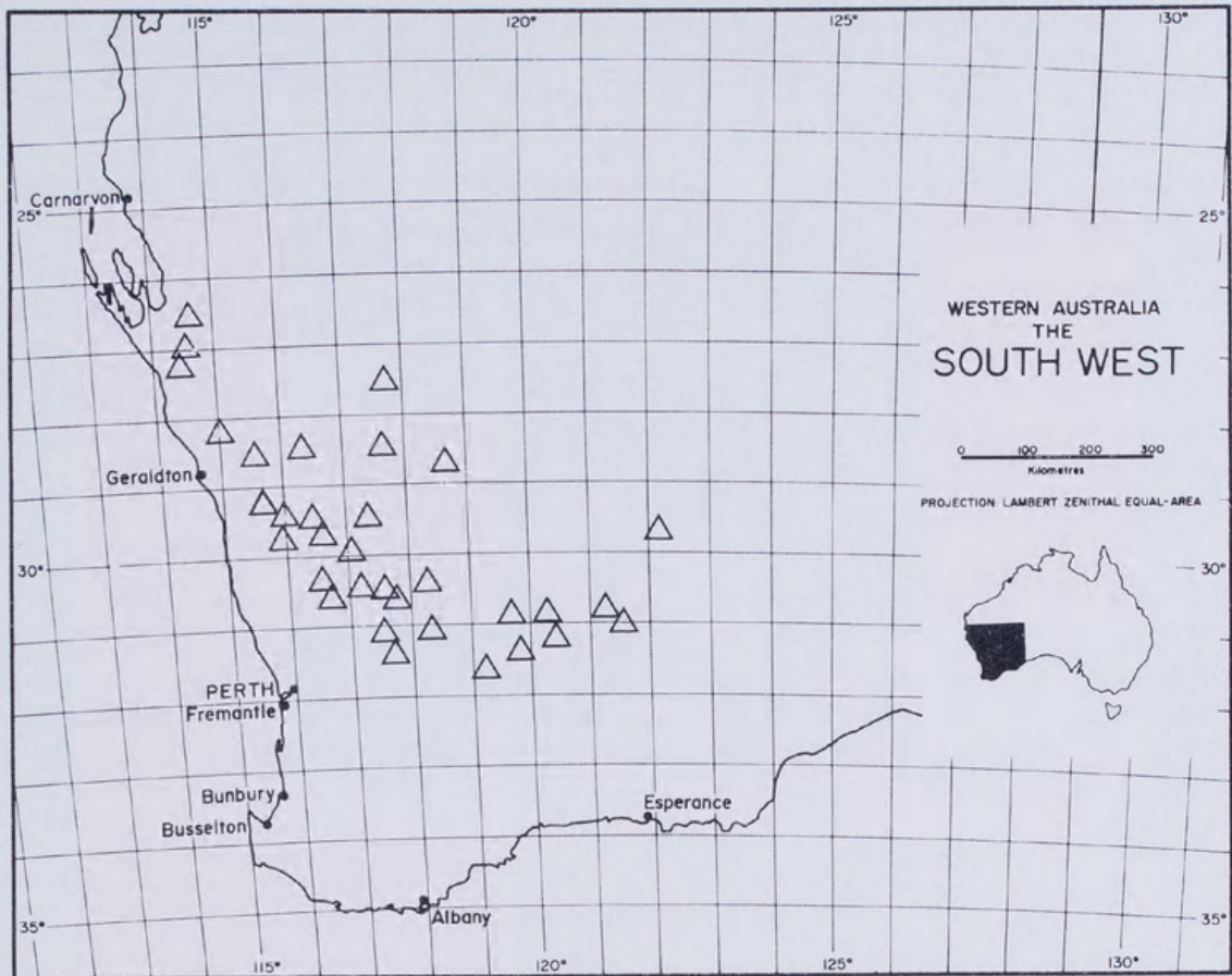
Map 3. Distribution of Malleostemon roseus .
