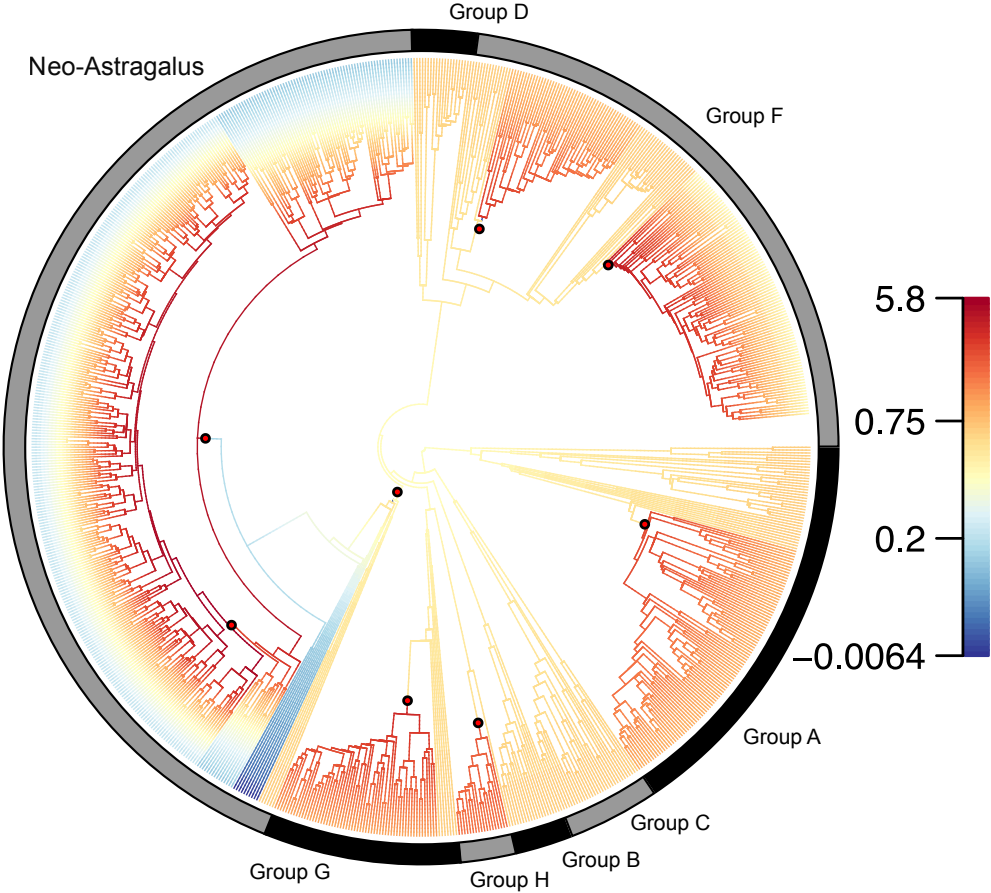
Fig. S2. Plot of BAMM net diversification rate shifts. Red dots indicate shifts in BAMM rate regime; branch colors represent net diversification per the legend, in events per million years.
