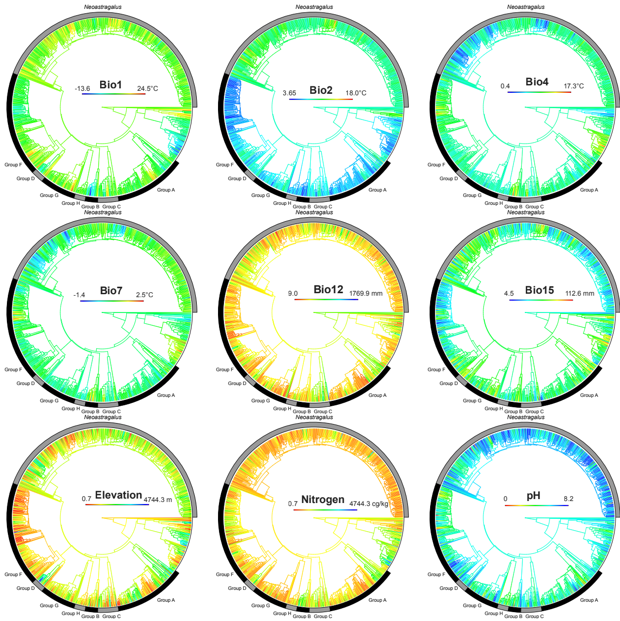
Fig. S3. Ancestral reconstructions for the 9 predictor variables not shown in the main text.
