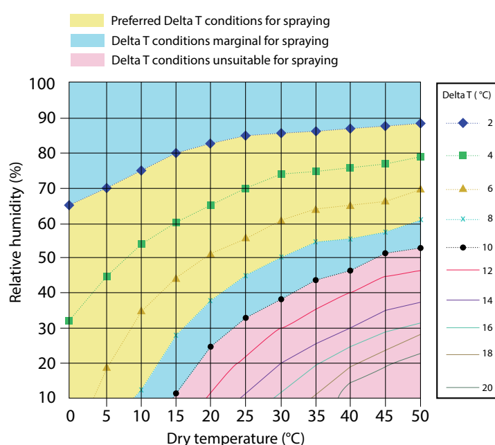
Figure 172. Delta T chart. Source: Bureau of Meteorology.
