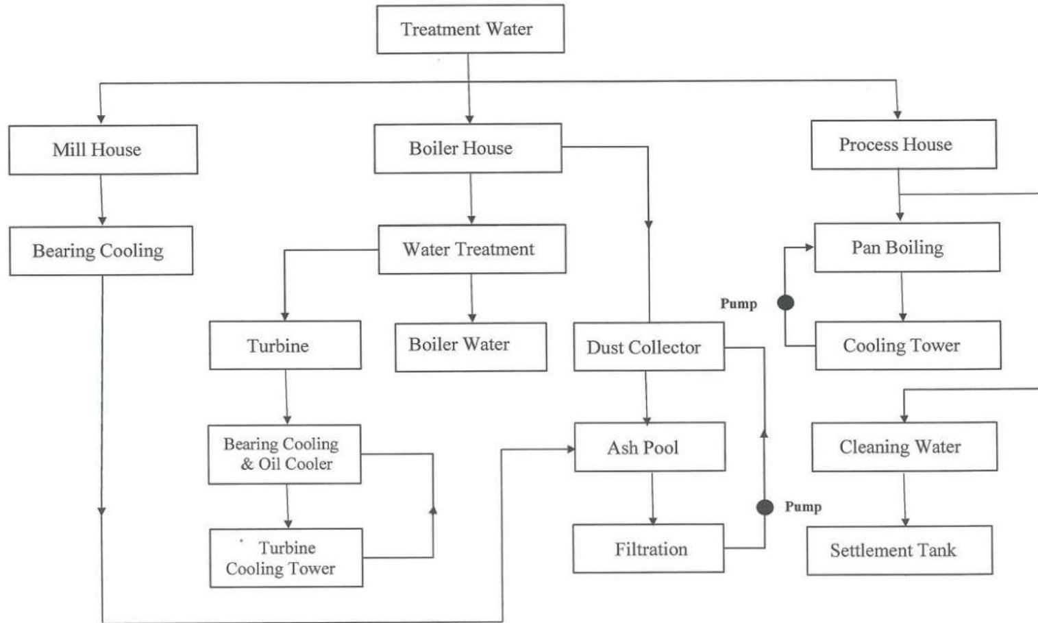
Figure – 31: Water usage system of the factory
