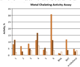
Figure. Antioxidant activity results and the structures of the tested compound.
