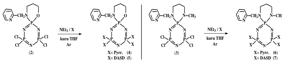
Figure 1. 2-Pyridylspirocyclotriphosphazene derivatives (4-7).
