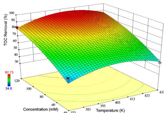
Figure 1. Variation of TOC removal rate of aniline based on the H_2O_2 concentration and temperature at fixed treatment time of 30 min.
