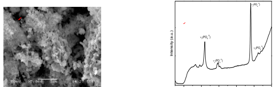
Figure 1. After biomimetic process (a) SEM image and (b) Raman spectrum of doped HA.
