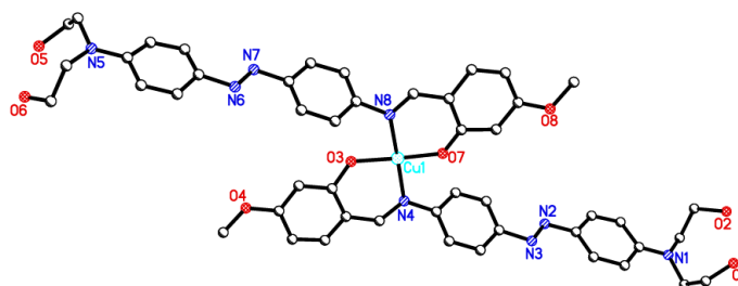
Fig. [Cu(L 7 ) 2 ] Molecular structure of the complex.
