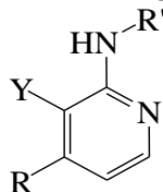
Figure 1: 2-aminopyridines structure
