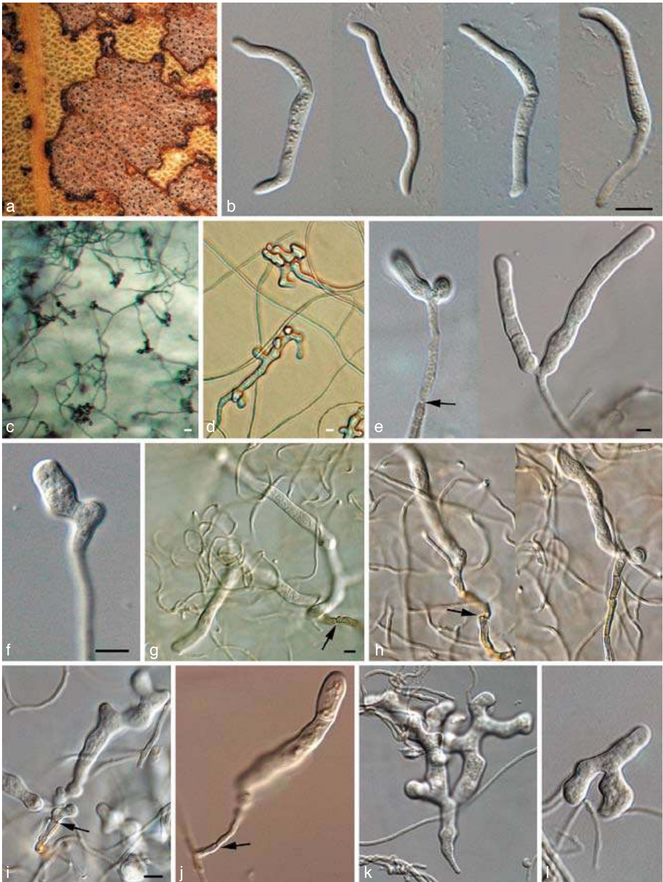
Fig. 21 Zasmidium arohyalinosporum (CPC 14636). a. Leaf spot with black spermatogonia (small black dots); b. germinating ascospores on MEA; c–l. conidiogenous cells giving rise to conidia (arrow denotes point of attachment). — Scale bars = 10 µm.
