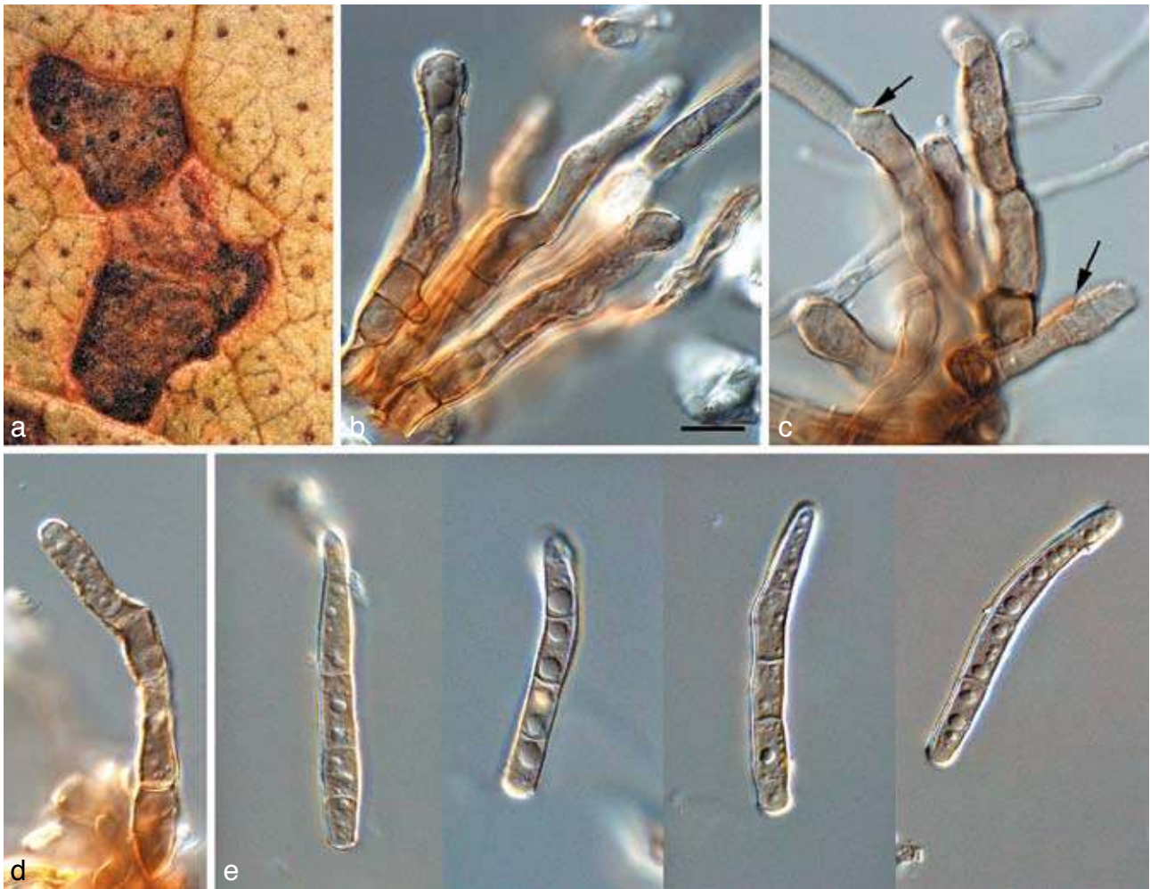
Fig. 8 Pseudocercospora tereticornis (CPC 13299). a. Leaf spots; b–d. conidiophores with conidiogenous cells (arrow indicates percurrent proliferation); e. conidia with guttules. — Scale bar = 10 \mu m.
