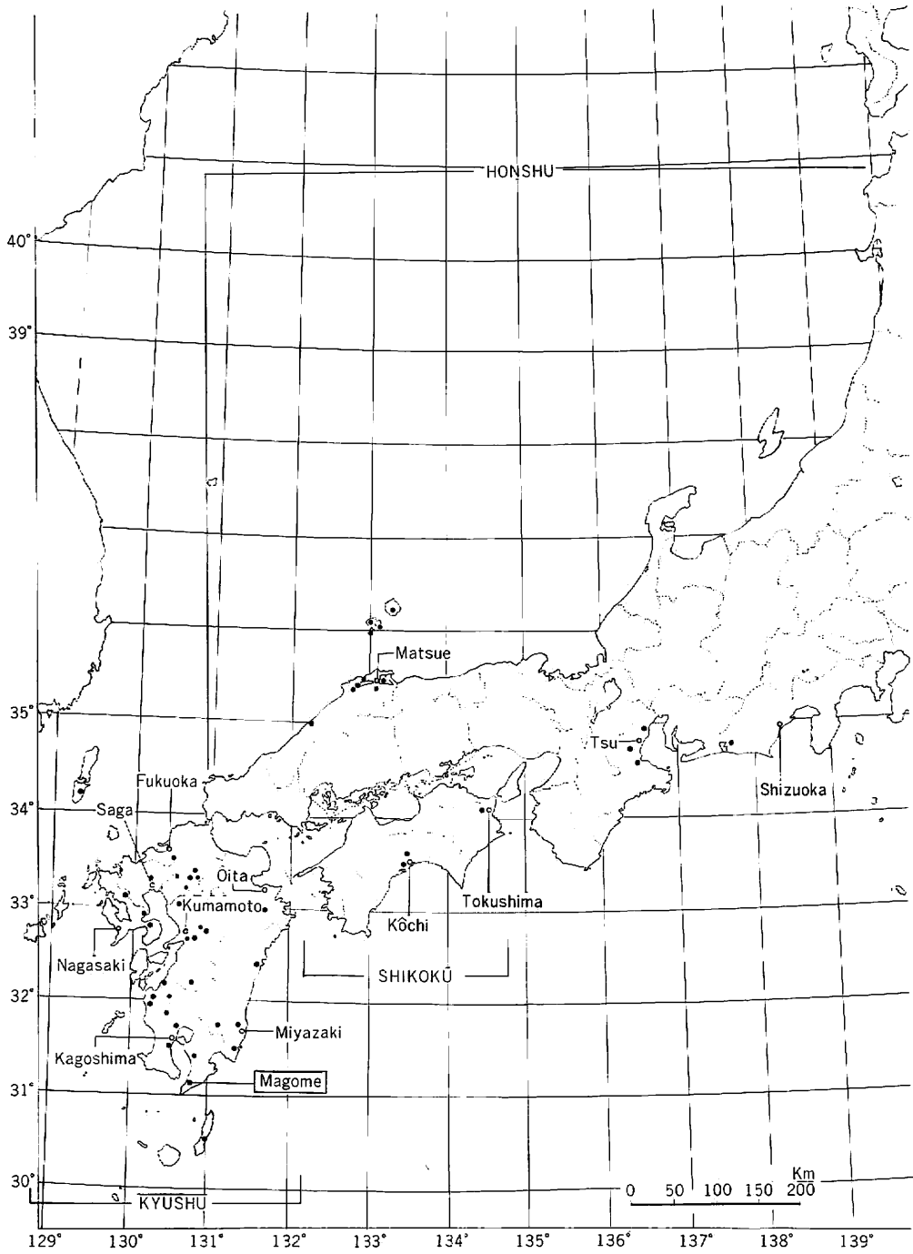
Fig. 3 Map of distribution of Cercospora pini-densiflorae in Japan.
