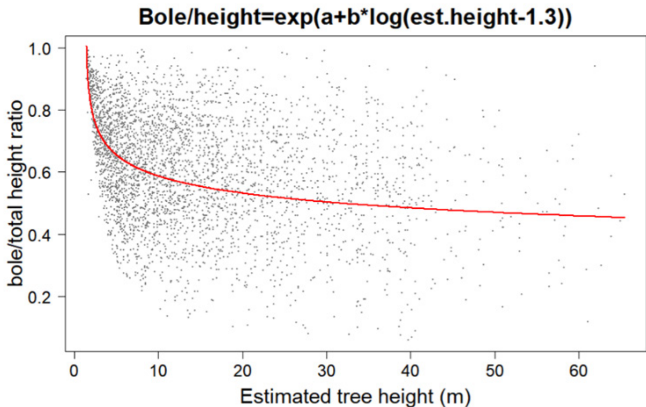
Figure 13. Bole to tree height ratio, modelled as a power function of height, where a,b <0. Observe that the equation above is an expanded version of that reported in the main text.
