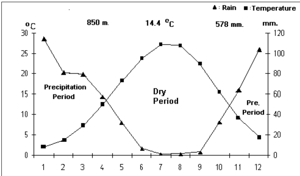
Fig. 2: Ombrothermic diagram of Gaziantep (for sources, see text).
