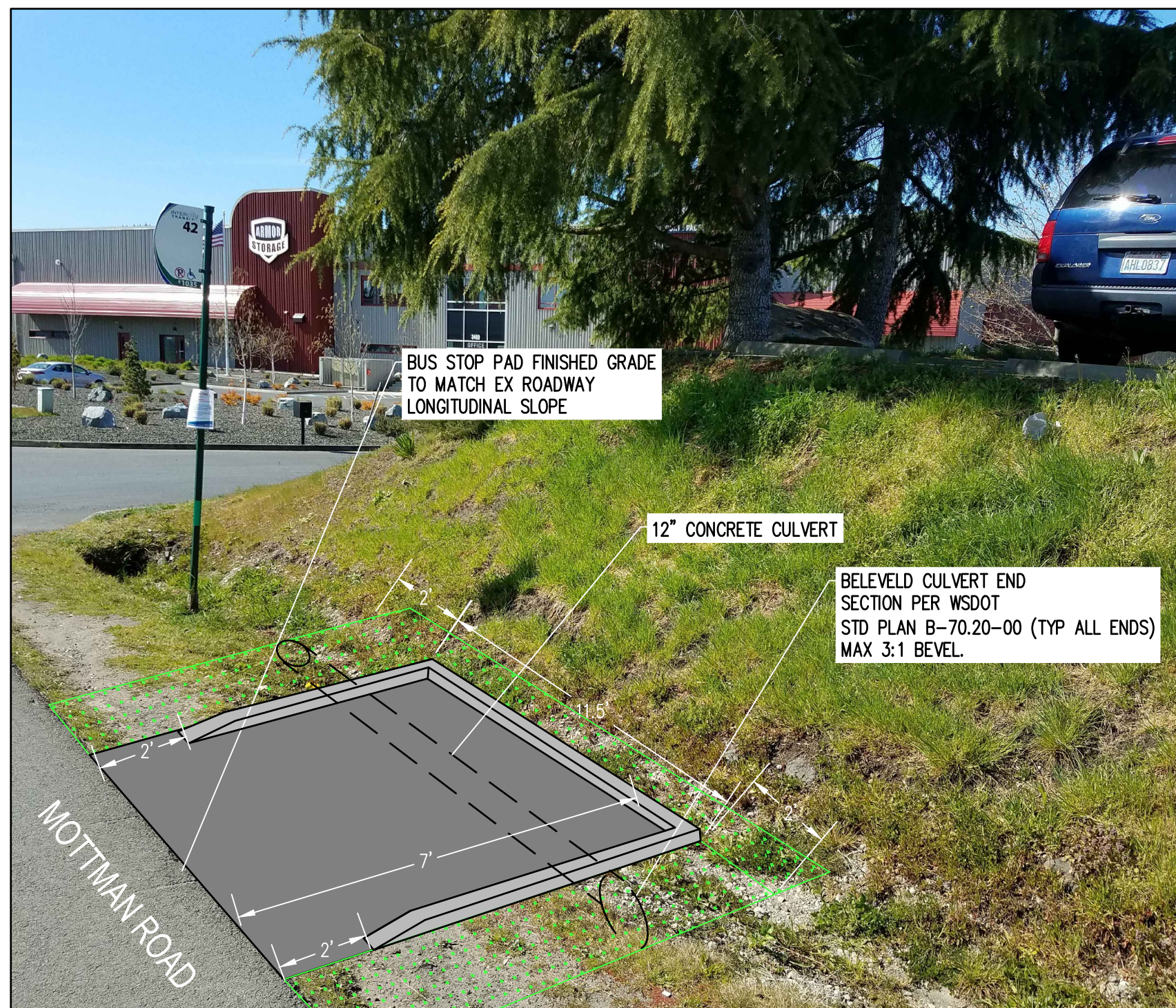
PROPOSED CONDITIONS N.T.S.
