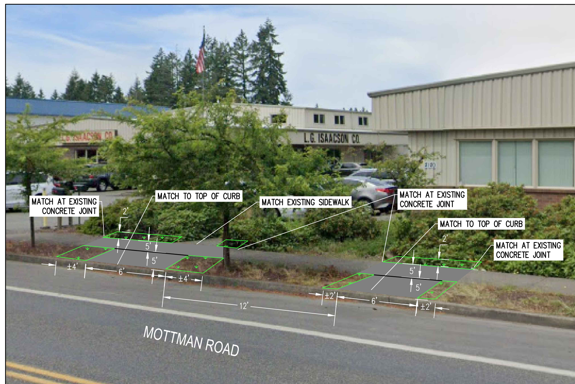
PROPOSED CONDITIONS N.T.S.
