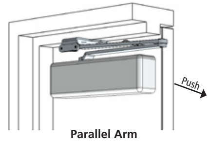
TYPICAL INSTALLATIONS (REGULAR ARMS SHOWN) Hold-Open Arms are similar
