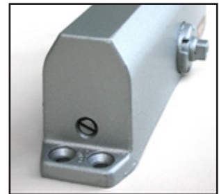
• 1803-BC, 1804-BC and 1805-BC Series Back-Check Adjustment Valve
