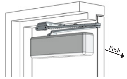
Parallel Arm (Push Side) Permits 180° maximum opening
