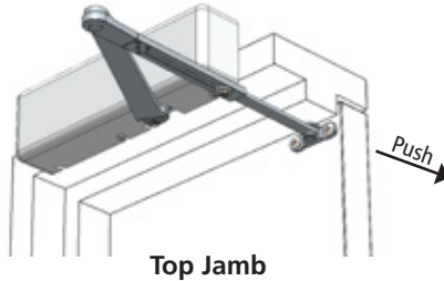
TYPICAL INSTALLATIONS (REGULAR ARMS SHOWN) Hold-Open Arms are similar
