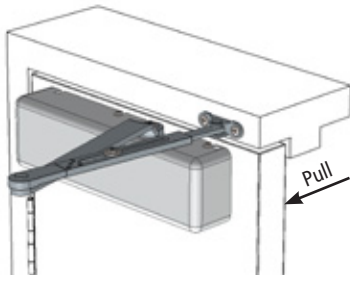
Regular Arm (Pull Side) Permits 120° maximum opening
