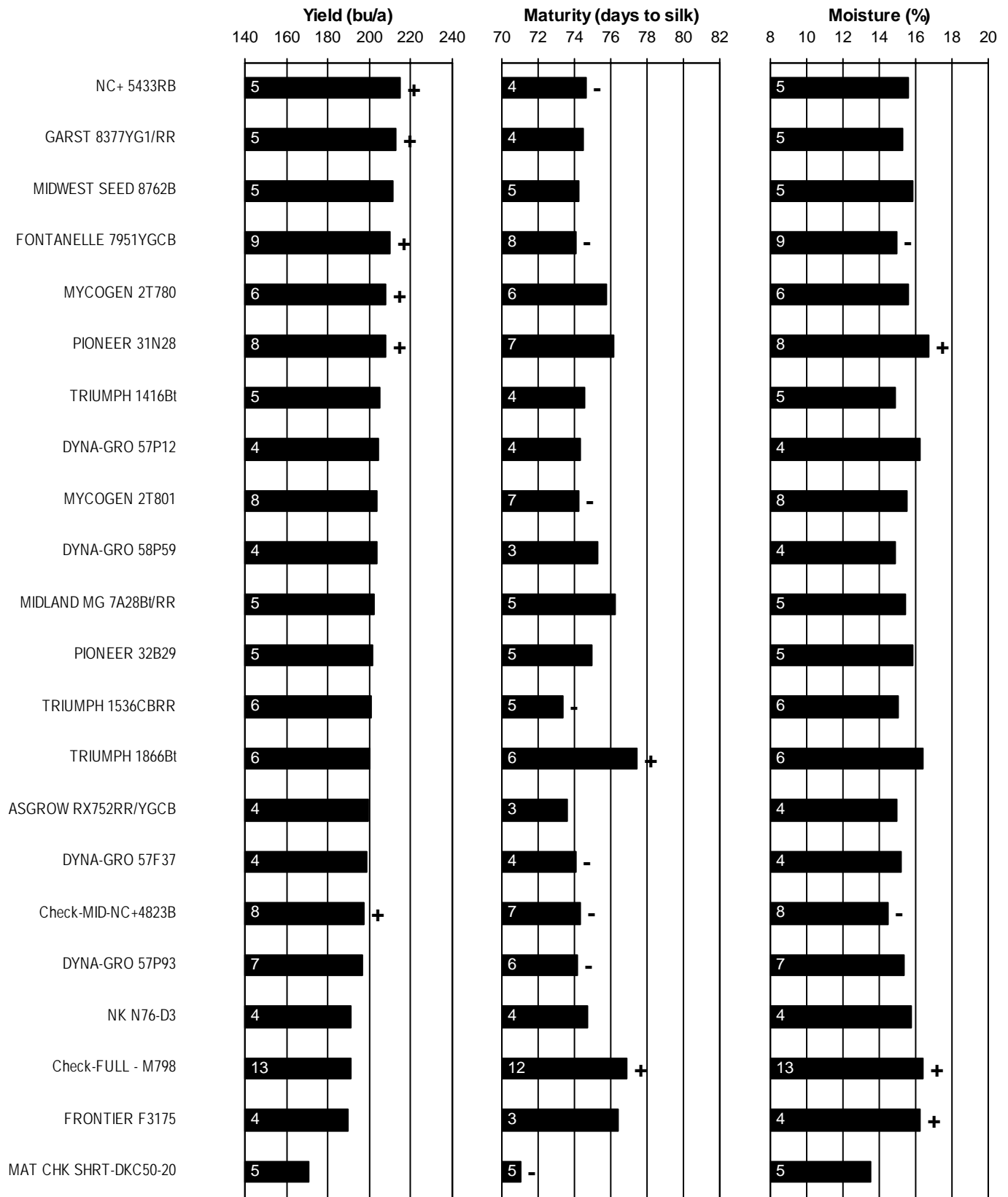
Figure 7. CENTRAL Kansas IRRIGATED corn hybrid standardized performance summary, 2002-2006.
