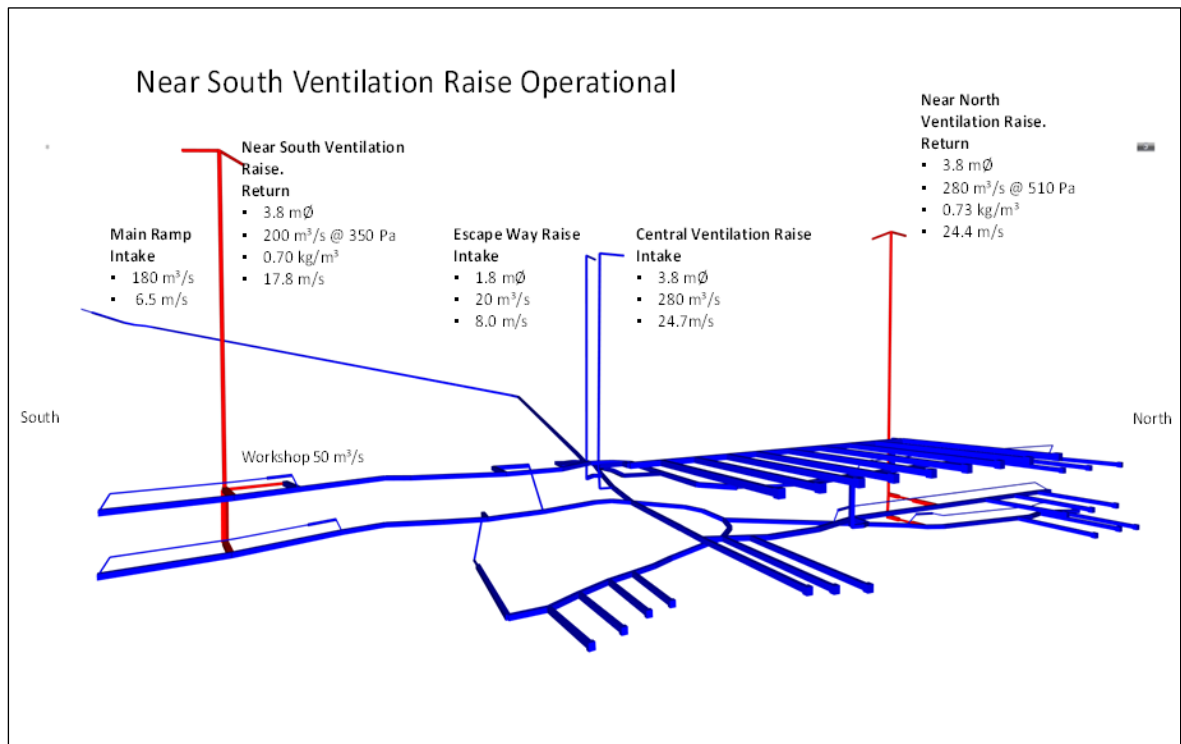
Figure 16-23: Near South Ventilation Raise Operational
