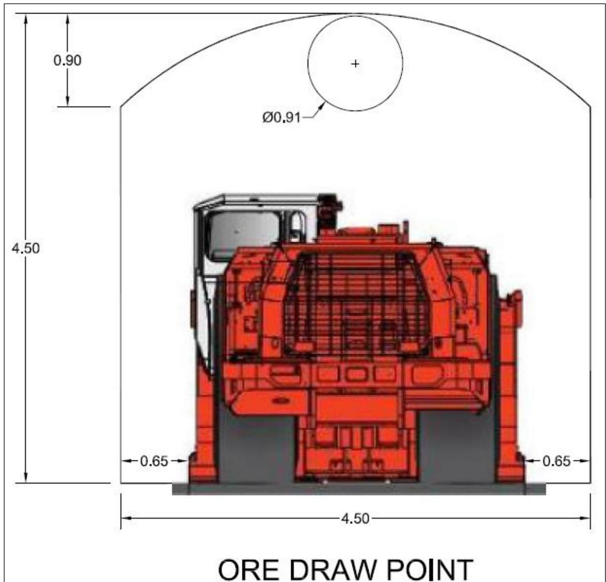
Figure 16-12: Drawpoints and Drilling Drift General Arrangement
