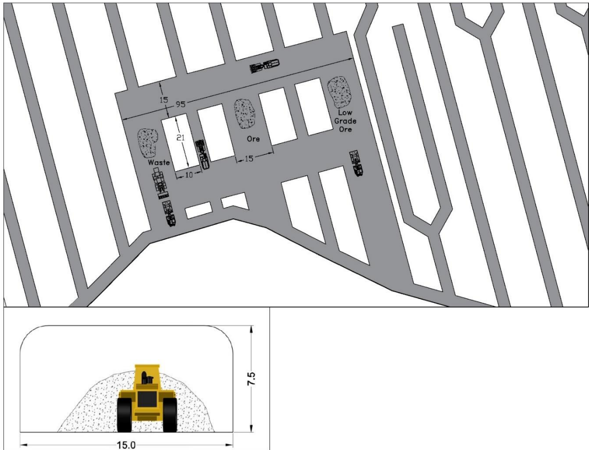
Figure 16-13: Loading Station - Plan View
