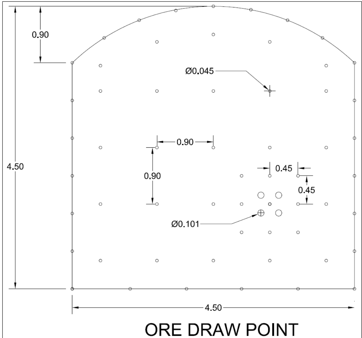
Figure 16-15: Drawpoint Drift Blast Drilling Pattern
