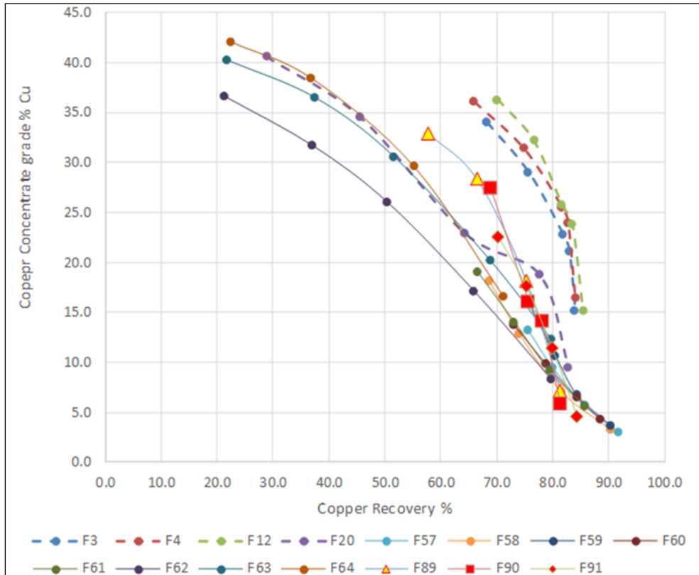
Figure 13-5: Copper Cleaner – Copper Grade vs Recovery
