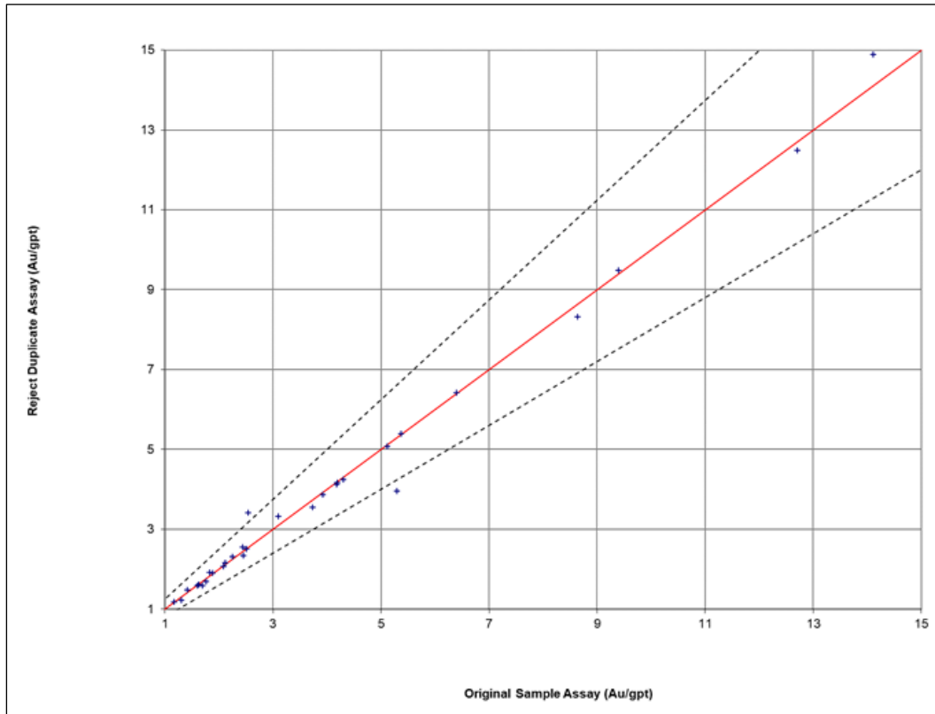
Figure 11-13: Gold Reject Duplicate Scatterplot
