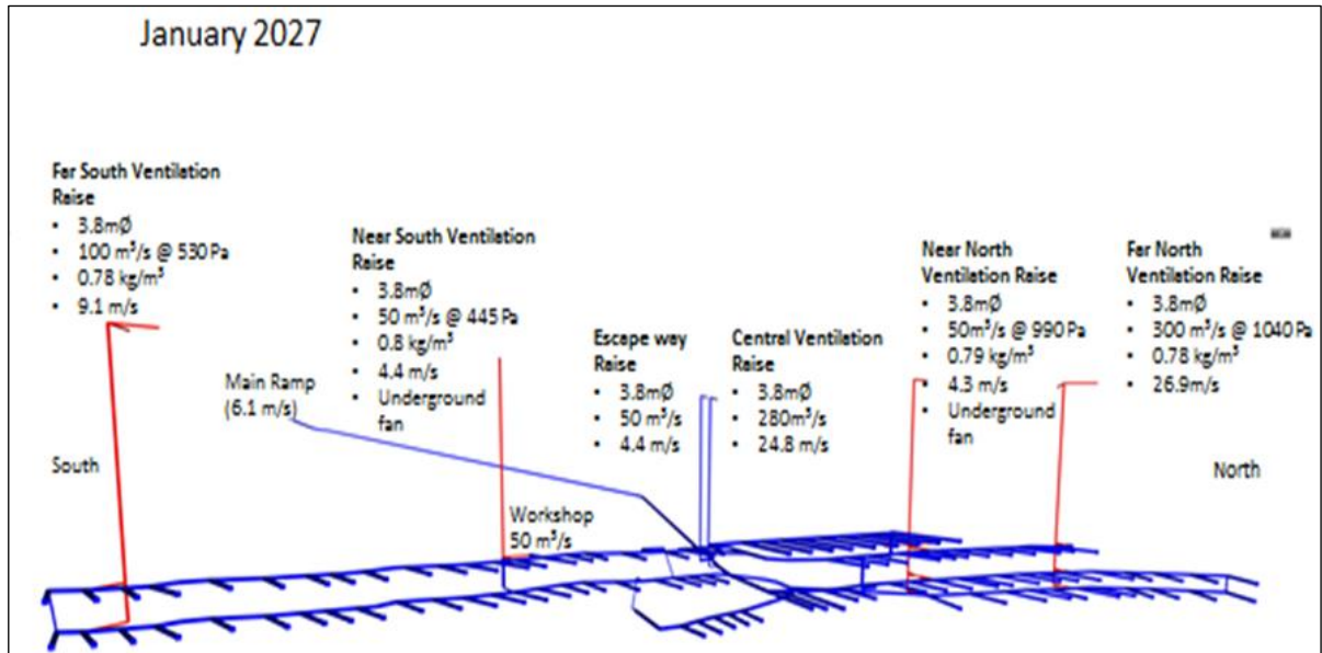
Figure 16-16: Main Ventilation Infrastructure
