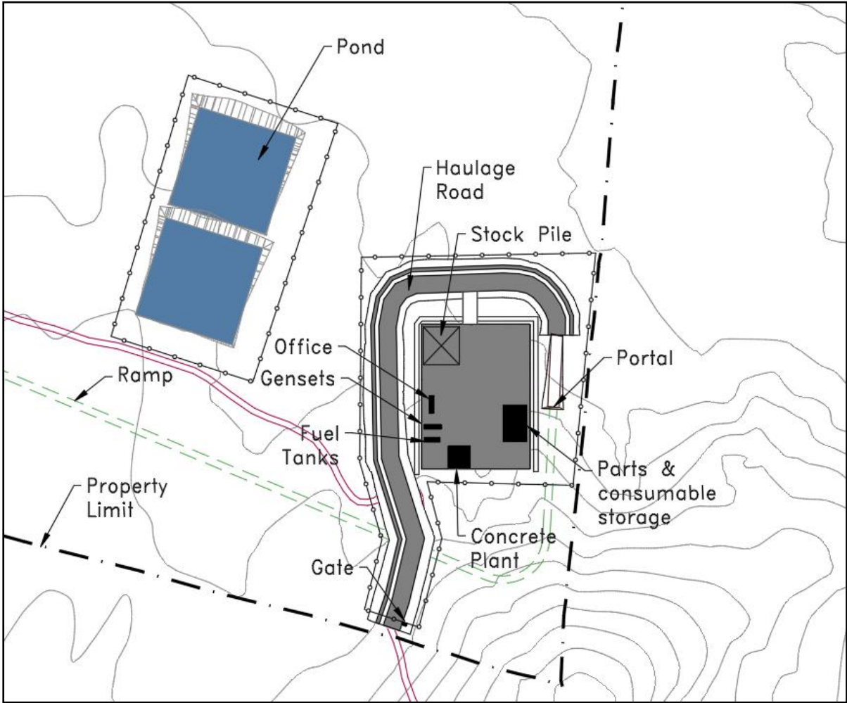
Figure 16-8: Portal Layout
