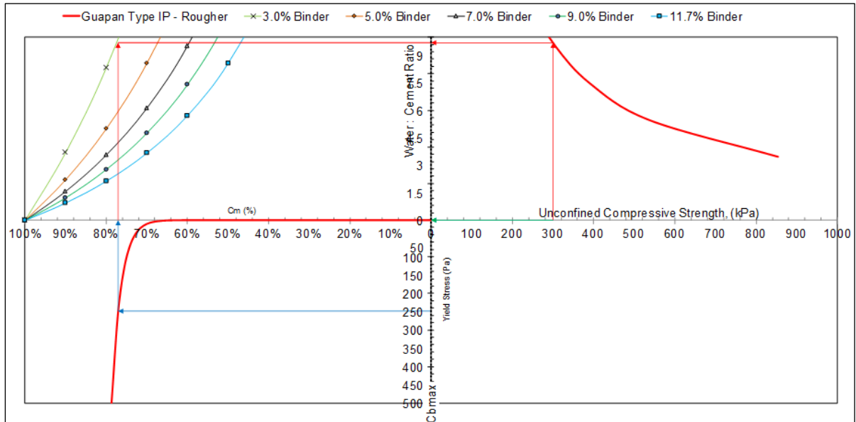
Figure 16-27: Binder Estimate (28 Day Target Strength)
