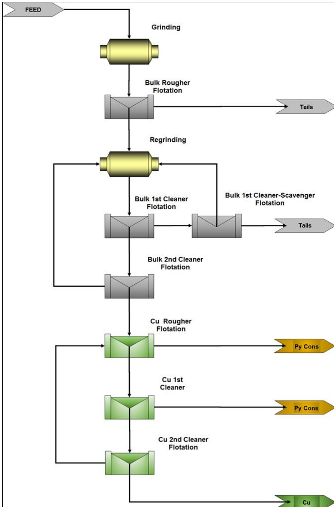
Figure 13-9: LCT #1 Flowsheet
