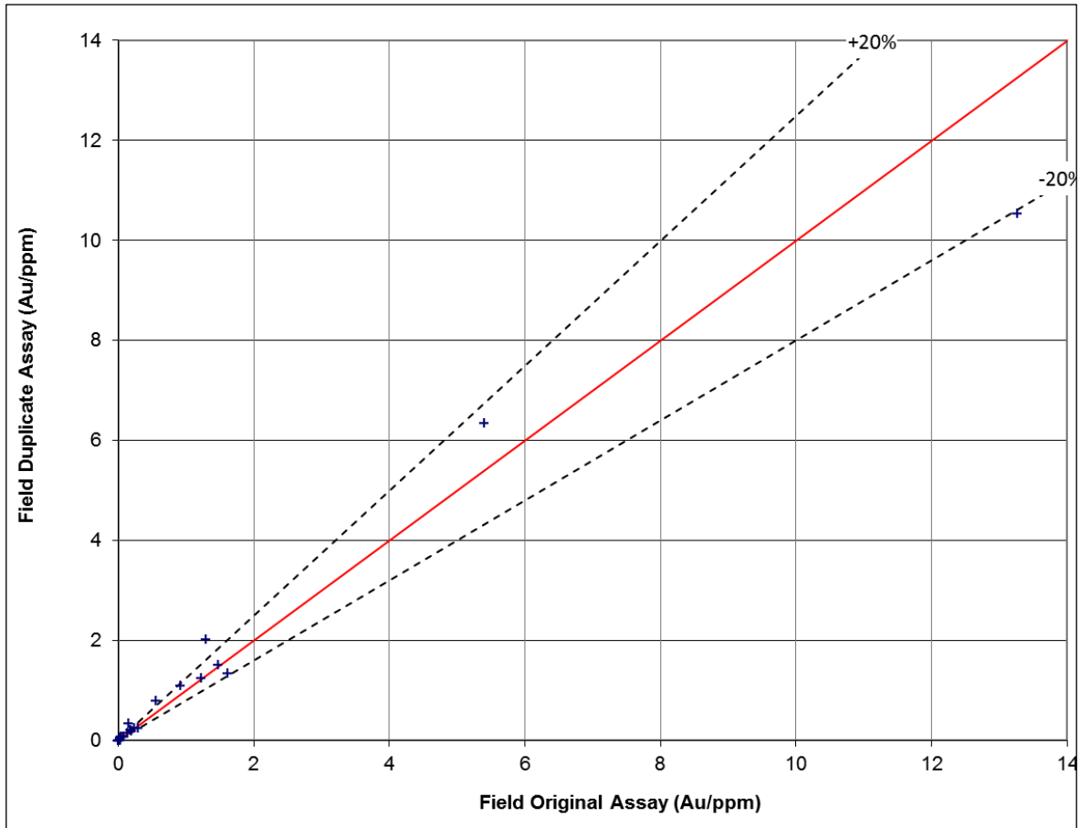
Figure 11-4: Gold Field Duplicate Scatterplot
