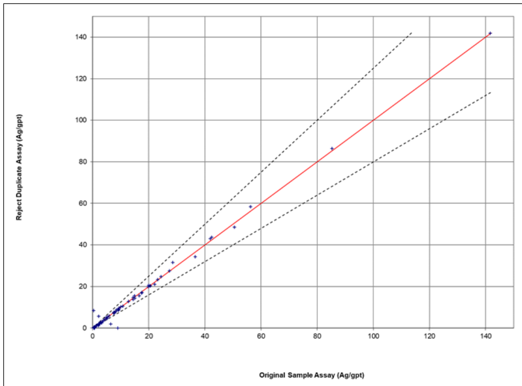
Figure 11-14: Silver Reject Duplicate Scatterplot
