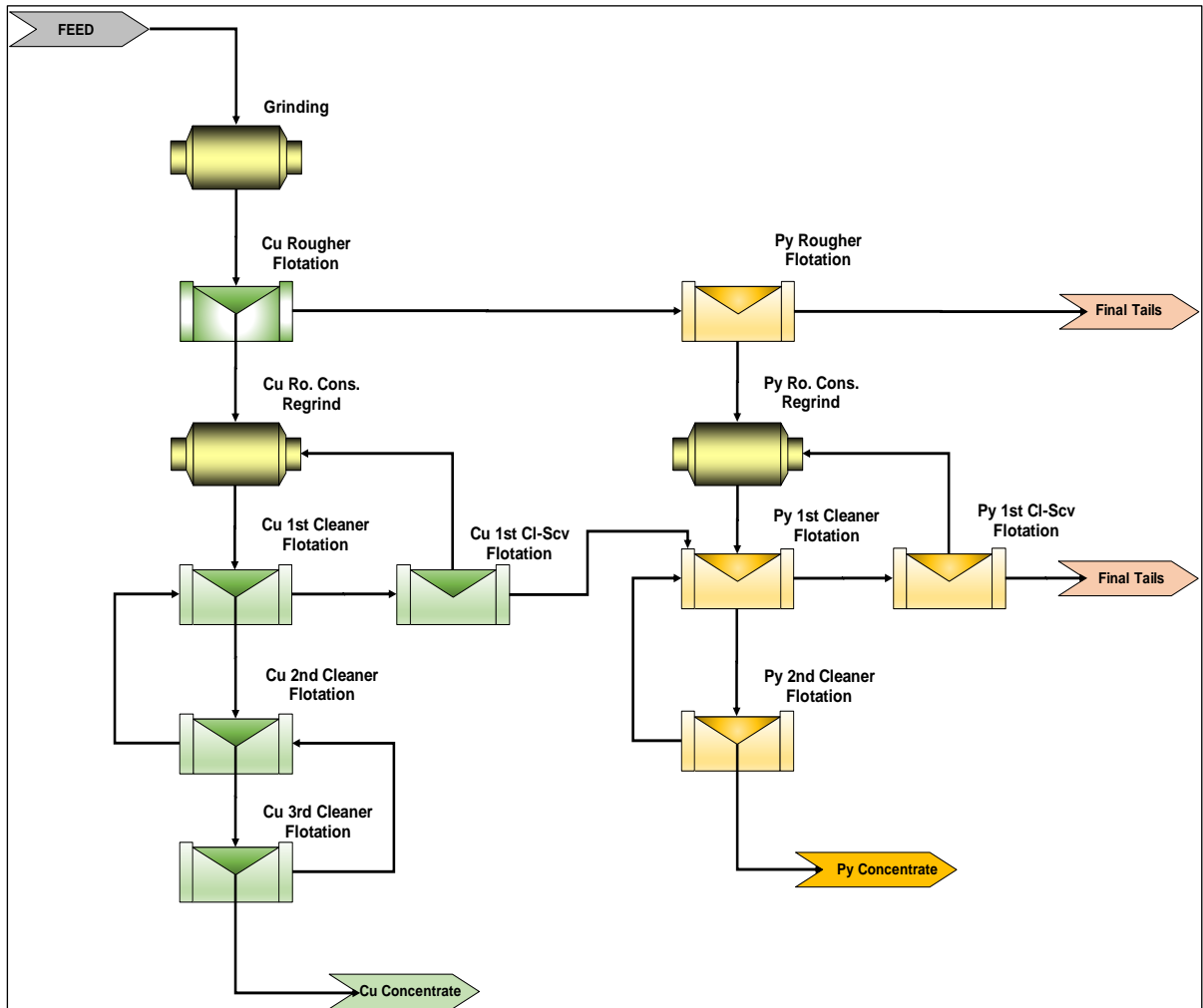
Figure 13-11: LCT #3 Flowsheet
