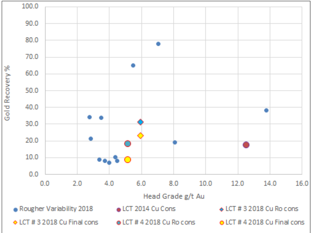
Figure 13-14: Gold Department to Copper Concentrates
