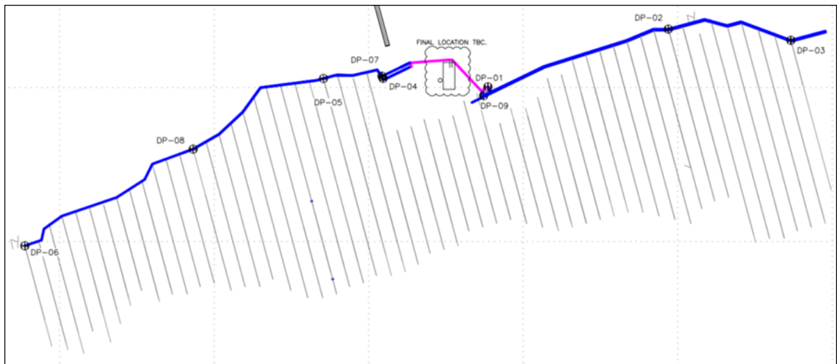
Figure 16-29: Schematic Diagram of Underground Workings – Pipeline Profile (Plan View)
