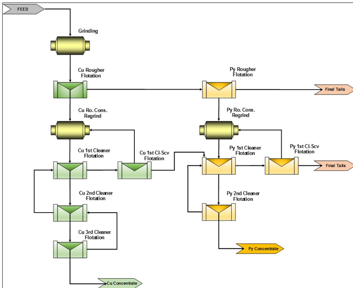
Figure 13-12: LCT #4 Flowsheet
