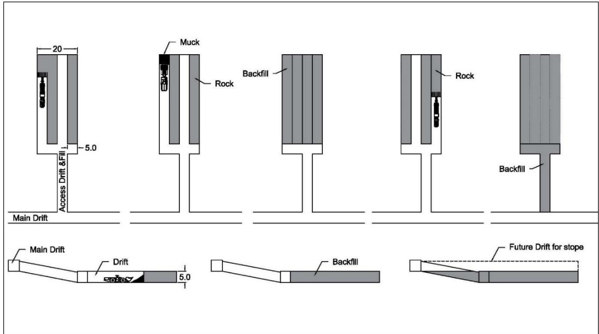
Figure 16-4: Drift and Fill Method
