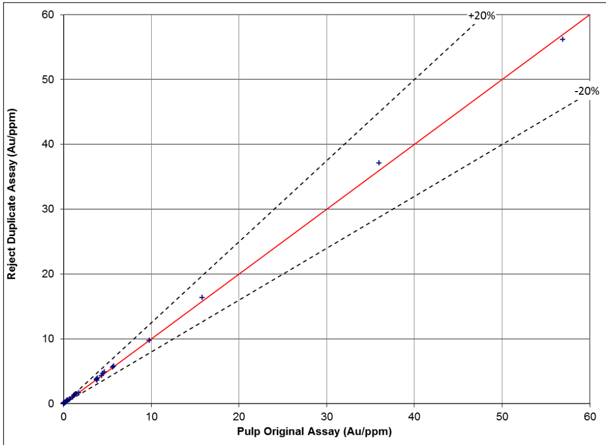
Figure 11-5: Gold Reject Duplicate Scatterplot
