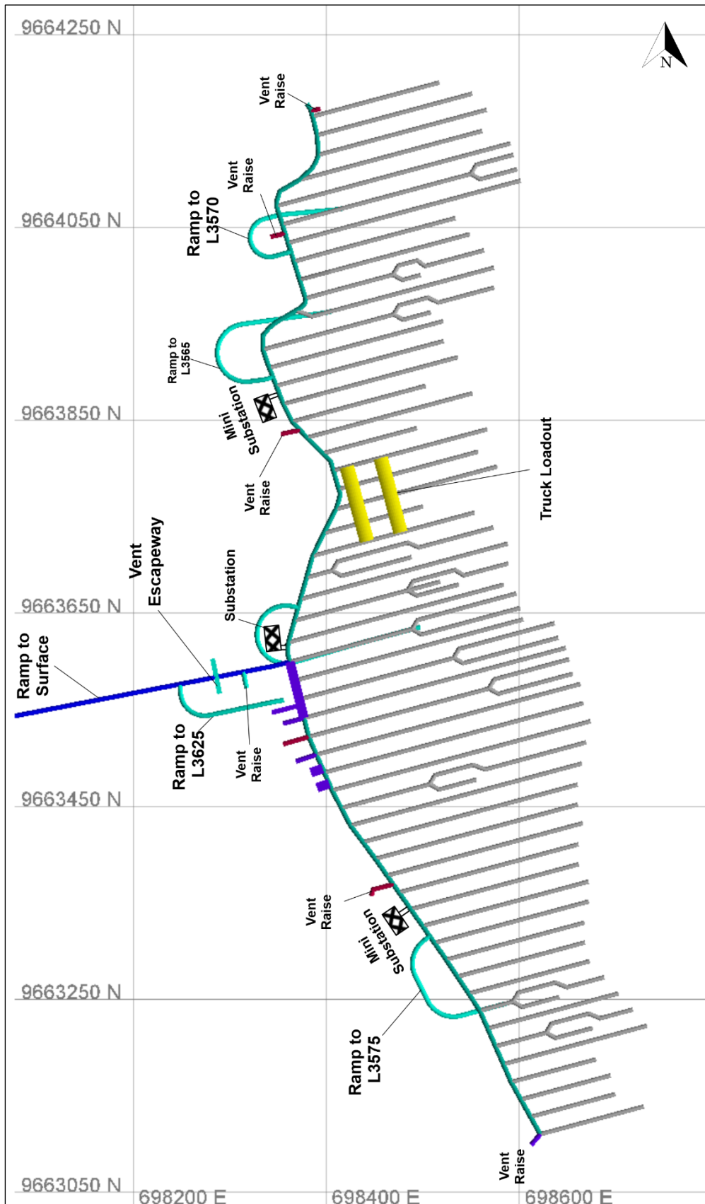
Figure 16-33: Level 3,600 Power Distribution
