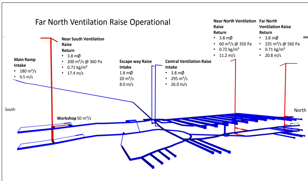
Figure 16-24: Far North Ventilation Raise Operational
