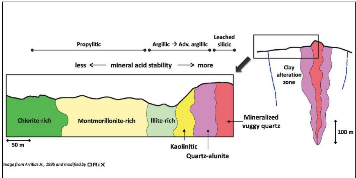
Figure 8-1: Zonation of Alteration in a High Sulphidation Deposit – After Arribas Jr. (1995)
