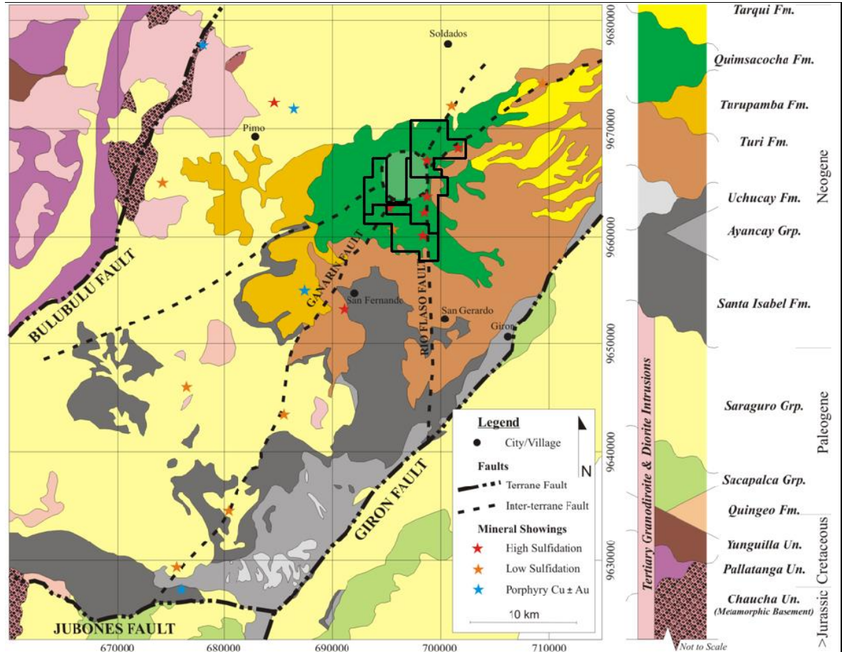
Figure 7-2: Regional Geology
