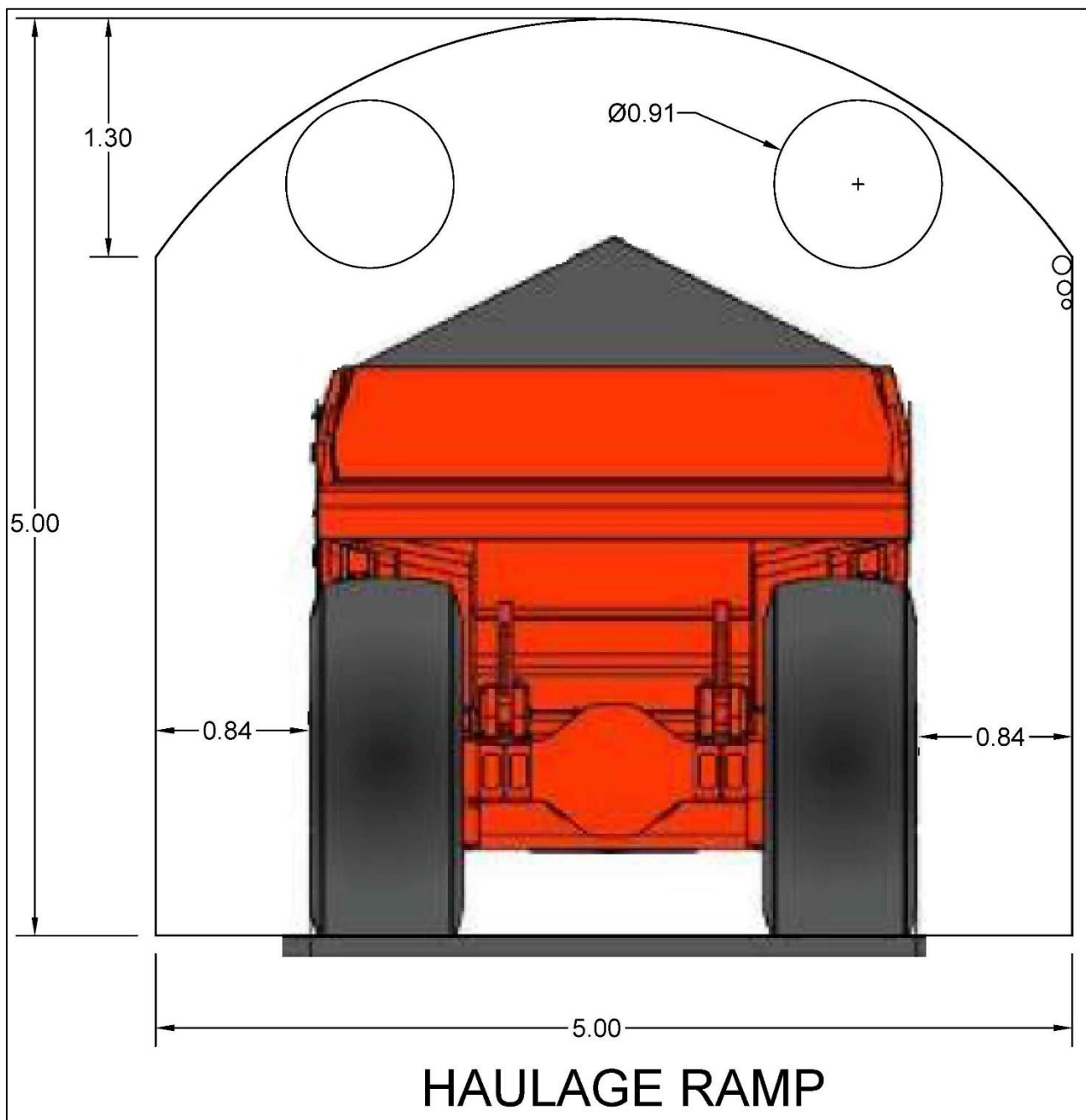
Figure 16-10: Haulage Ramp General Arrangement with 40-ton Truck
