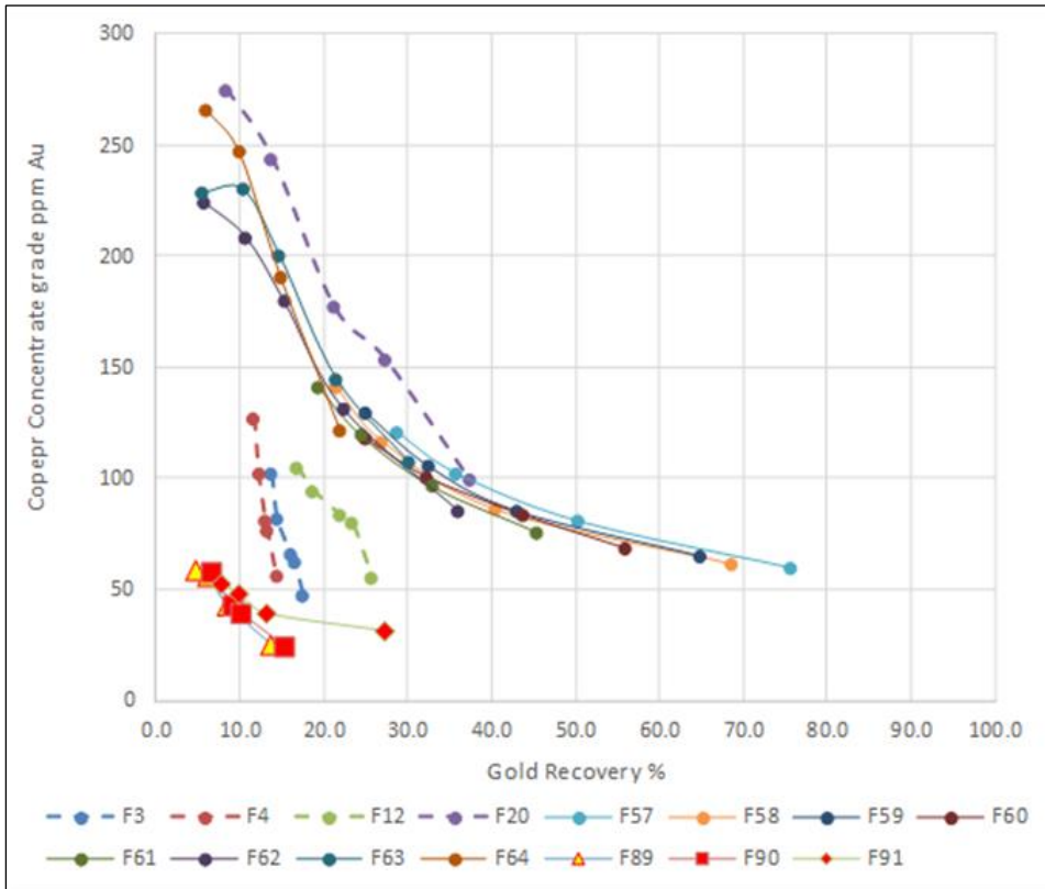
Figure 13-7: Copper Cleaner Gold Grade vs Recovery
