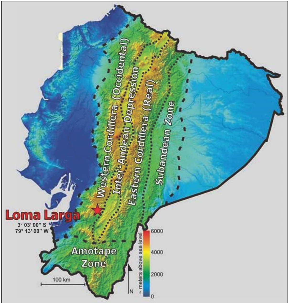
Figure 7-1: Major Terranes of Ecuador – Source: Modified from MacDonald et al., SEG September 25, 2013 Whistler
