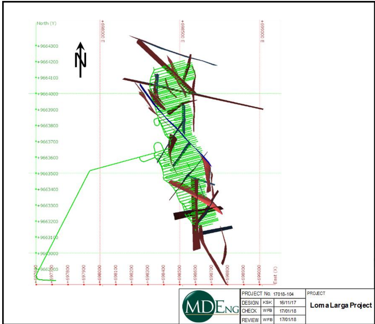
Figure 16-7: Large-Scale Structural Features
