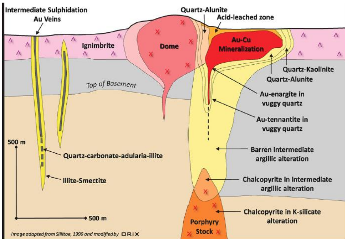
Figure 8-2: Schematic Section of a High Sulphidation Deposit – After Sillitoe (1999)
