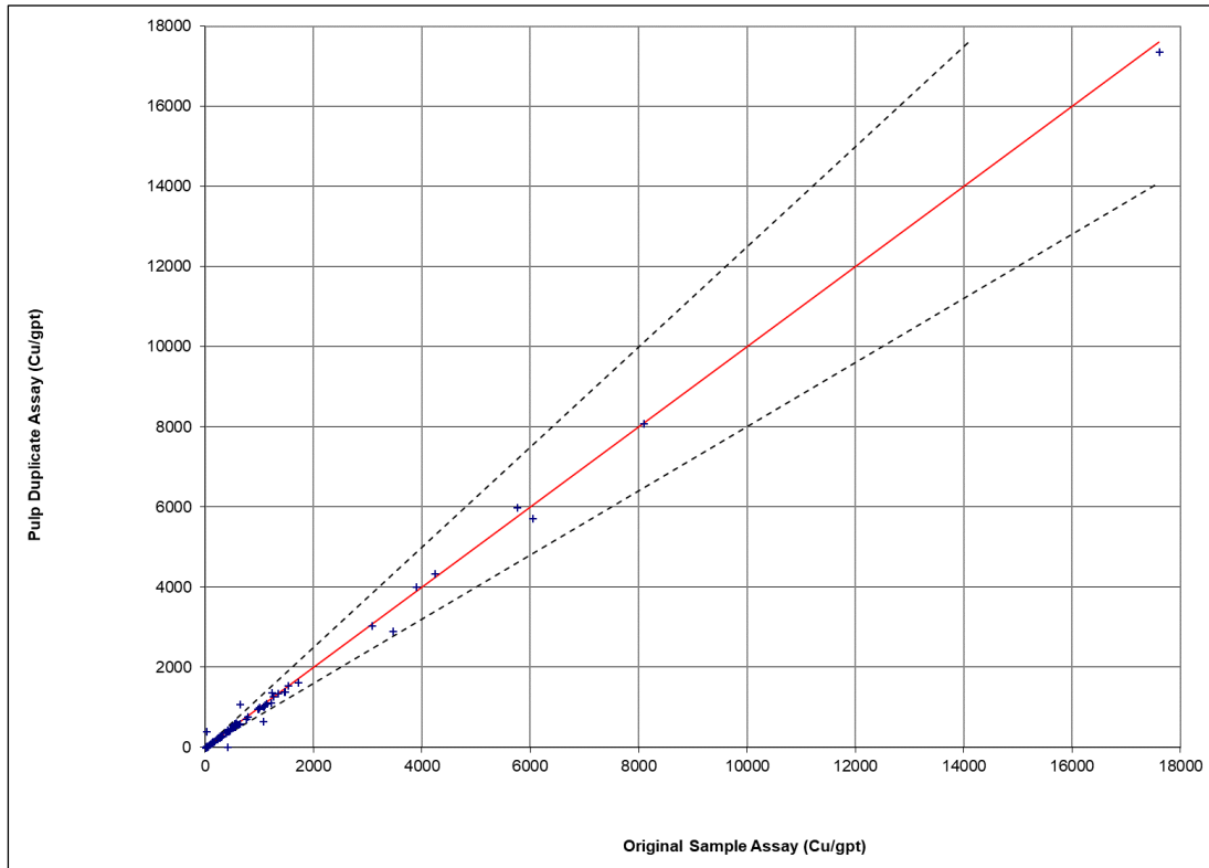
Figure 11-18: Copper Pulp Duplicate Scatterplot
