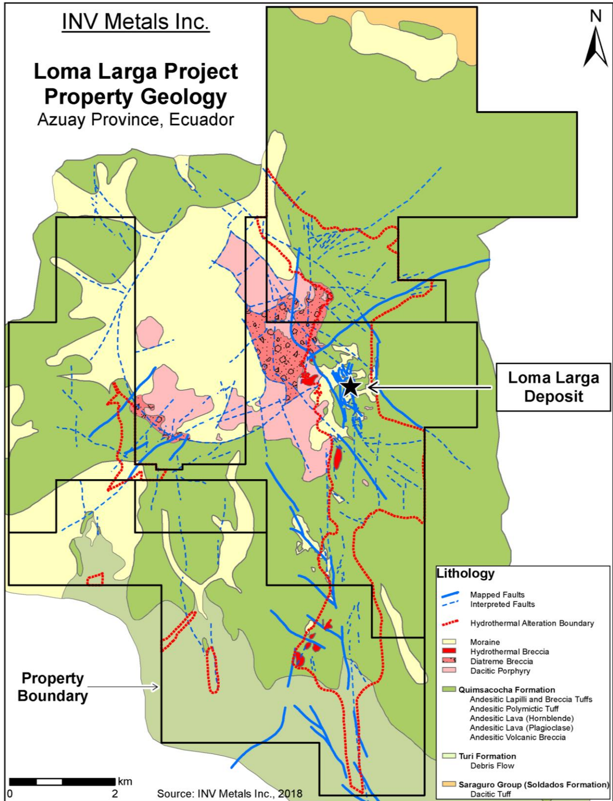
Figure 7-3: Property Geology
