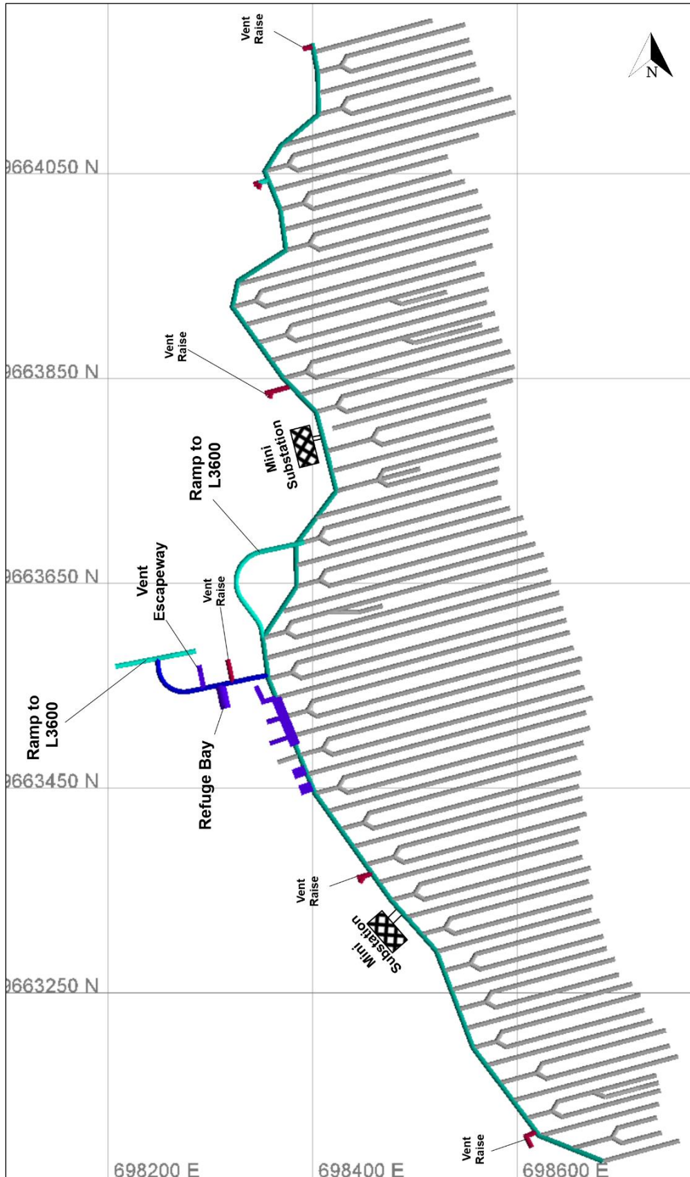
Figure 16-34: Level 3,625 Power Distribution
