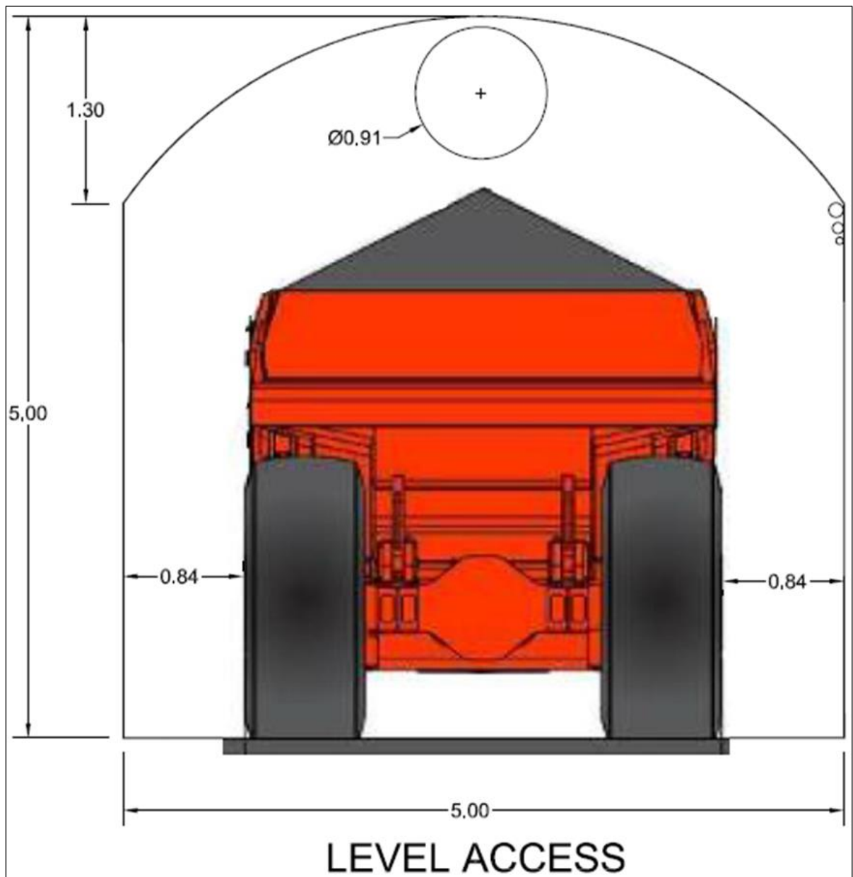
Figure 16-11: Level Access General Arrangement with 40-ton Truck
