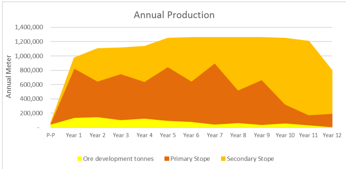
Figure 16-17: Extraction Profile
