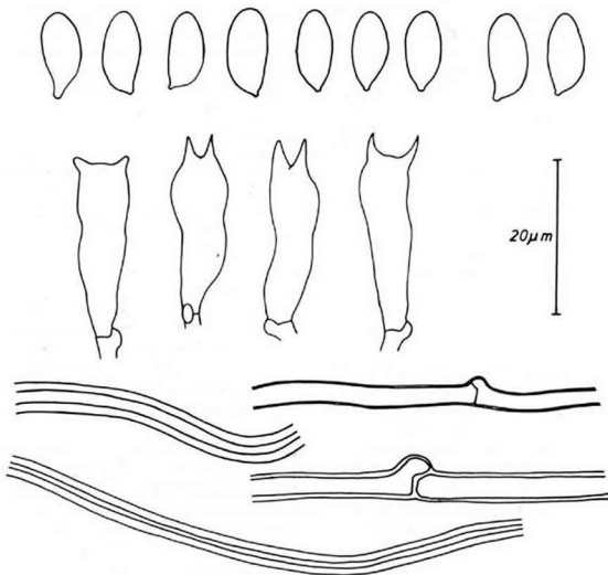
Fig. 1. Mucronella rickii Oud. — Holotype: spores, basidia, generative and skeletal hyphae.
