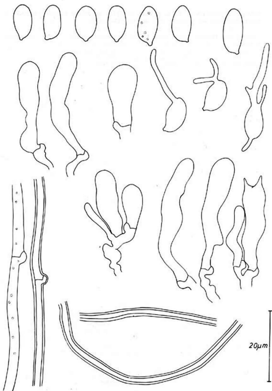
Fig. 2. Pterula gracilis . — Bas 2446a: spores, germinating spores, basidia, generative and skeletal hyphae.
