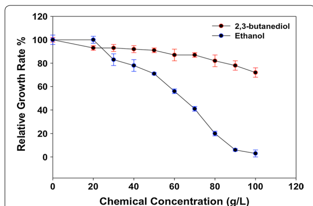
Fig. 1 The impact of meso -2,3-BDO and ethanol supplementation on growth of Z. mobilis in RMG medium at 30 °C using Bioscreen C. Relative growth rate (%) is the percentage of growth rate with chemical supplementation compared to control without
