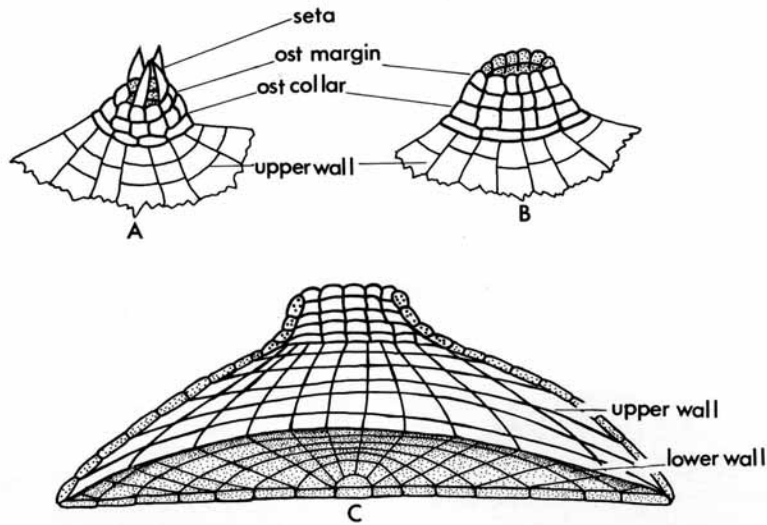
TEXT-FIG. 1. Diagrammatic representations of thyriothecium constructions in Trichothyriaceae. A, ostiole bearing setae on ostiolar margin. B, ostiole with smooth ostiolar margin. C, vertical section of the thyriothecium showing 3D structure. ost = ostiolar.
