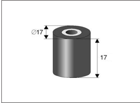
RODILLO, Interior Ø 4mm
