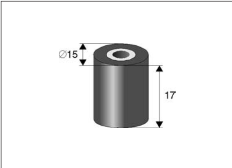
PR 022 RODILLO, Interior Ø 4mm
