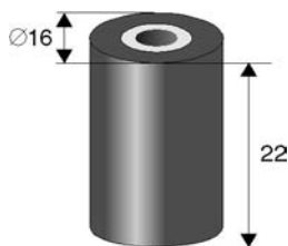
PR 005 RODILLO, Interior Ø 3mm
