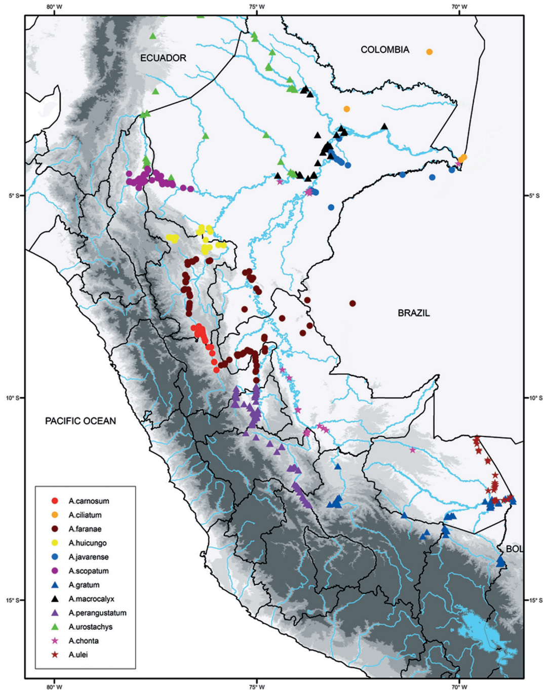
Figure 1. Distribution of Astrocaryum sect. Huicungo (Arecaceae) in Peru.
