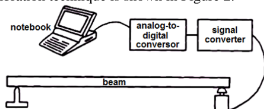
Figure 2. A simple setup for strength grading of timber by transversal vibration frequency.
