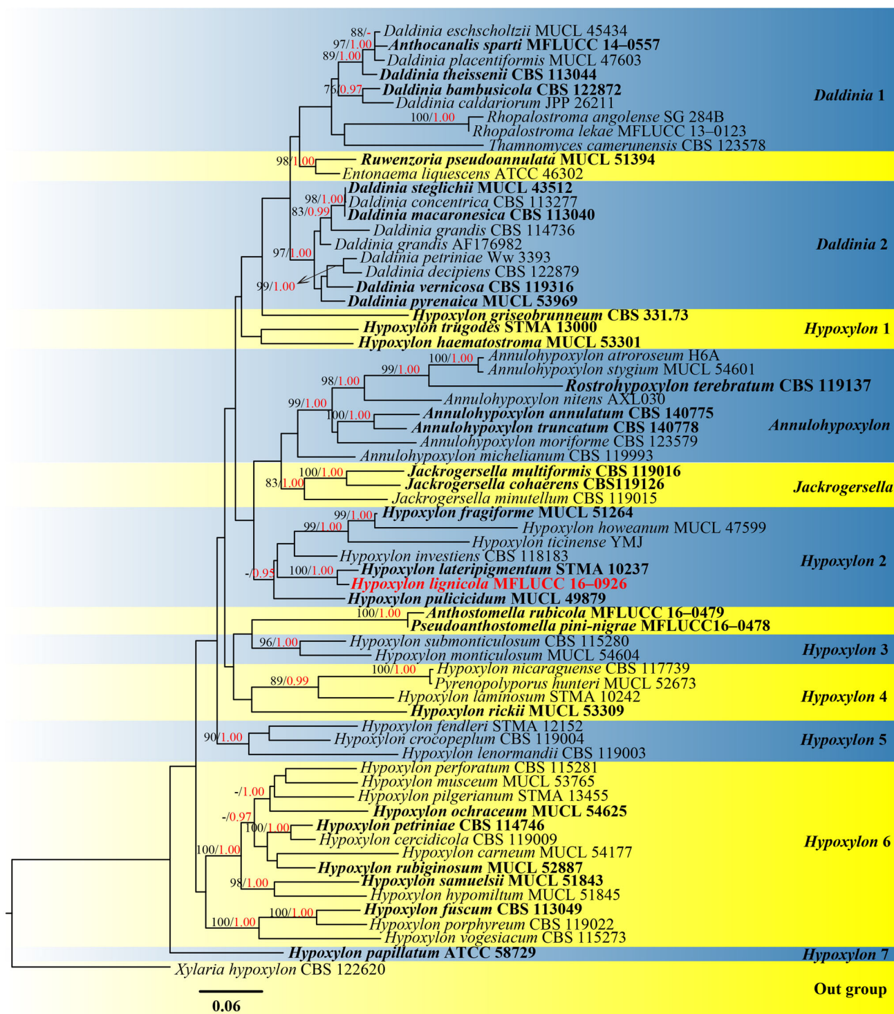
Fig. 77 Phylogram generated from maximum likelihood analysis based on ITS sequence data for species of Hypoxylaceae (with Xylaria hypoxylon as outgroup). The best scoring RAxML tree with a final likelihood value of -30247.954400 is presented. RAxML bootstrap support values equal to or greater than 75% are given before
