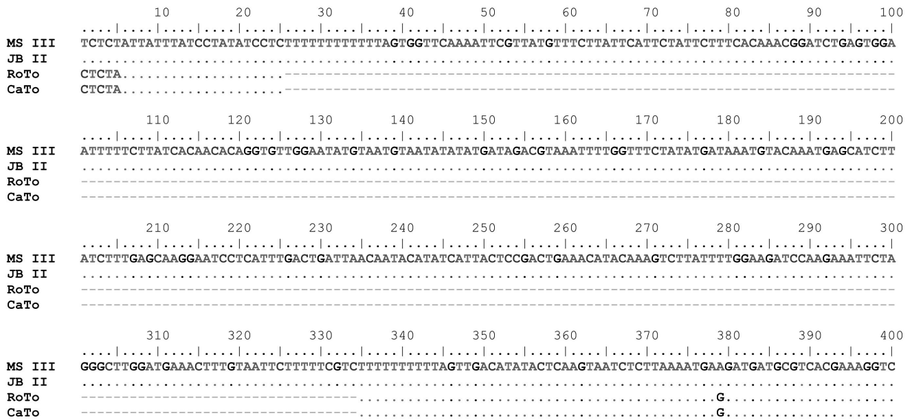
Figure 3. Sequence alignment of a section of the trnL-F gene in four exemplars of Inga showing the large indel in exemplars of the coastal plains (Roto and CaTo). MS III and JB II were collected from the mountainous region.
