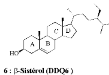
Figure 2: Molecular structures of triterpenoids isolated from R. vinei tubers
