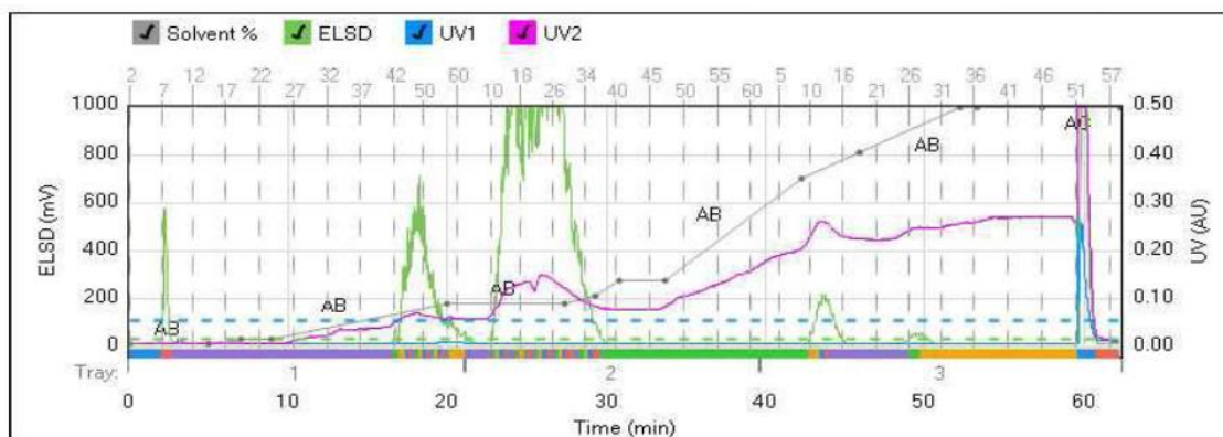
Figure 1: Flash REVELERIS purification chromatogram
