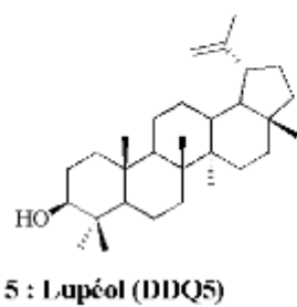
Figure 2: Molecular structures of triterpenoids isolated from R. vinei tubers
