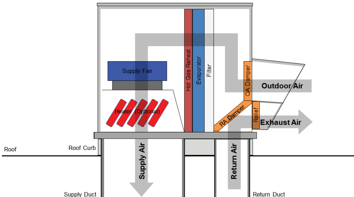
48/50LC*H with Economizer and Barometric Relief — 100% Outdoor Air Operation
