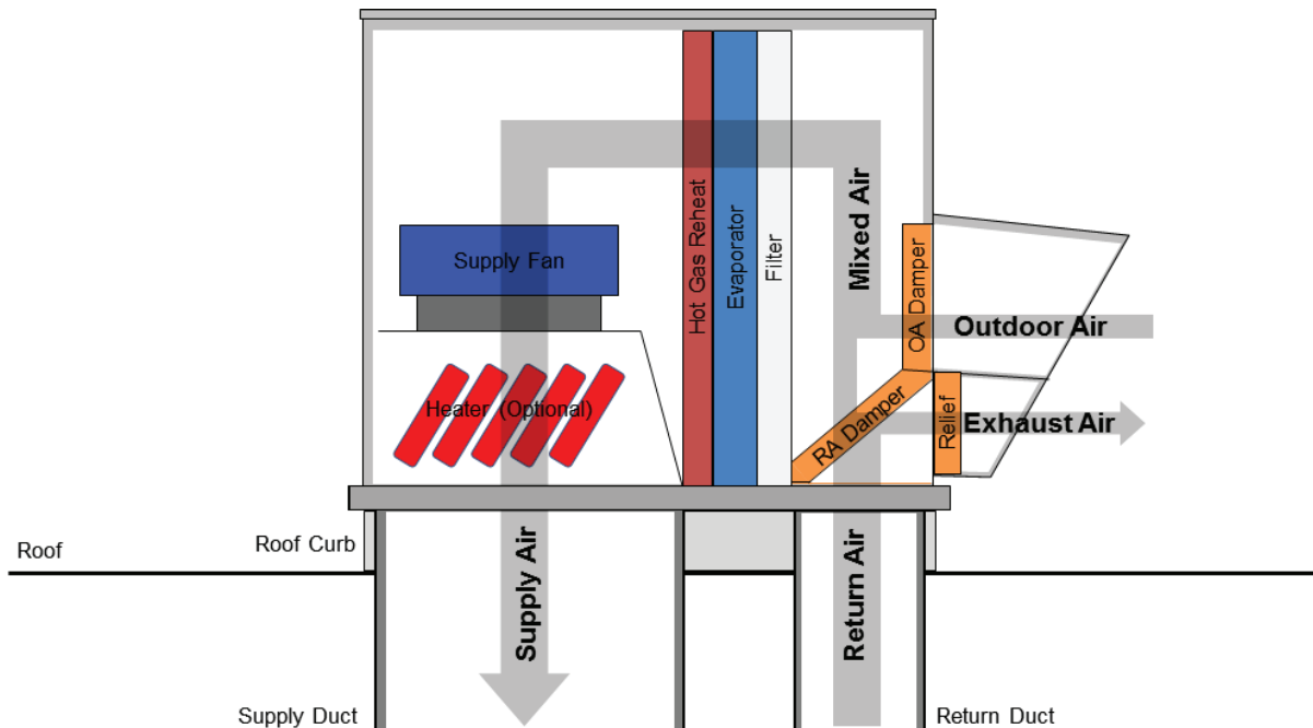
48/50LC*H Airflow Side View — Mixed Air with Economizer and Barometric Relief
