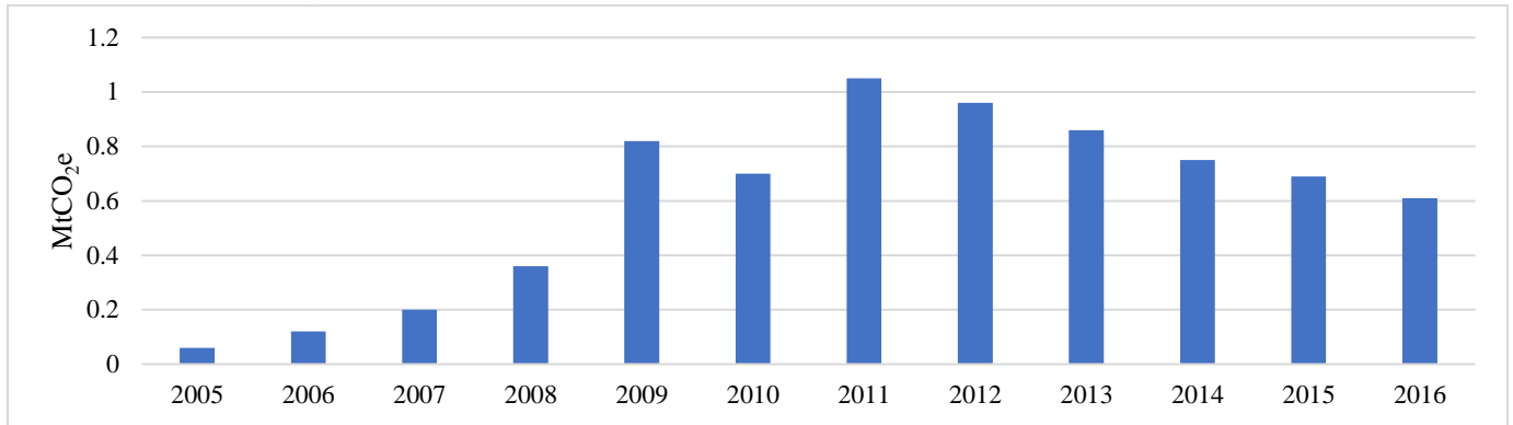
Figure 4.5: Annual Hydro fluorocarbon emission in MtCO 2 e
